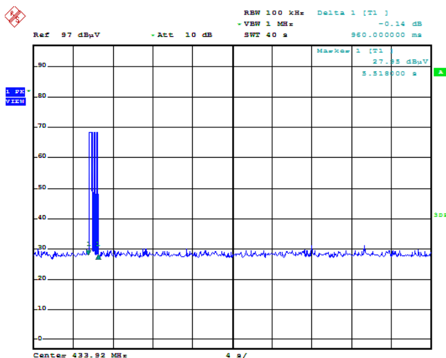
Transmission Time (ASK)
