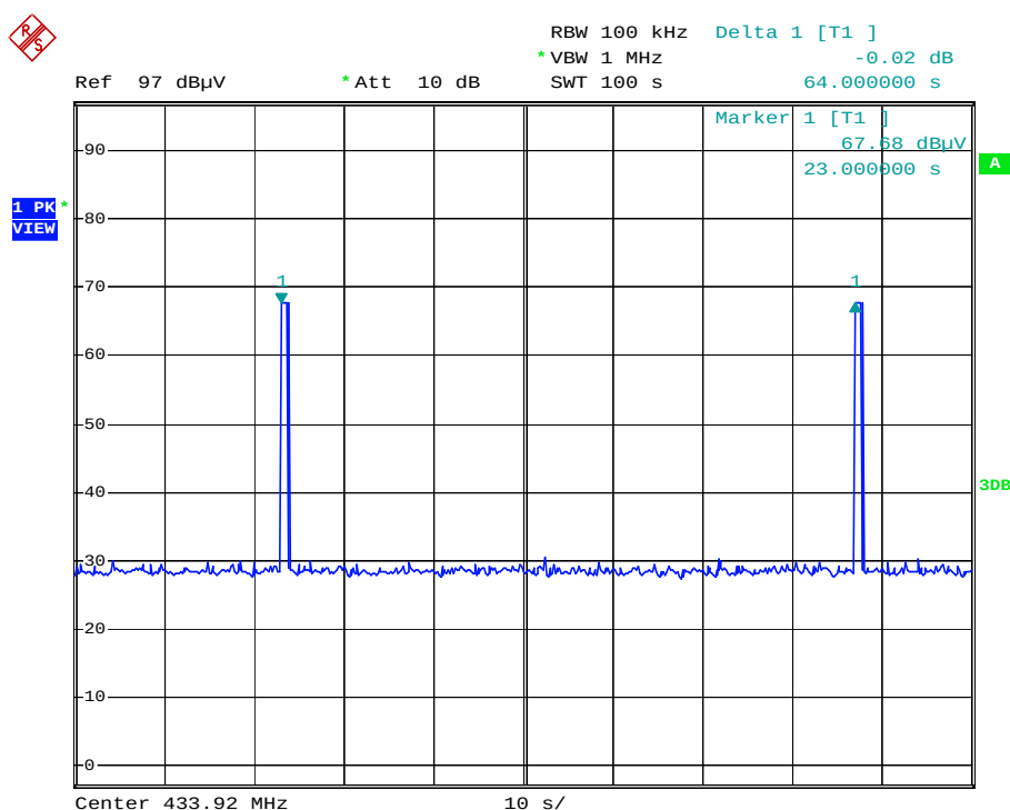
Transmission Period (ASK)
