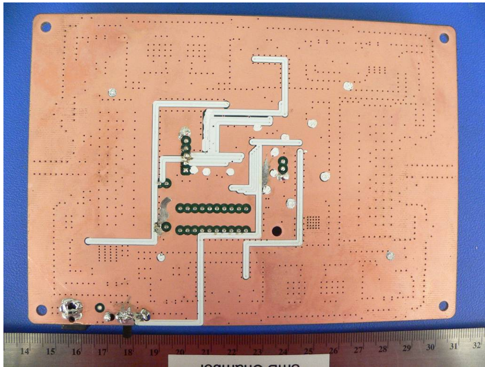
EUT – solder side view
