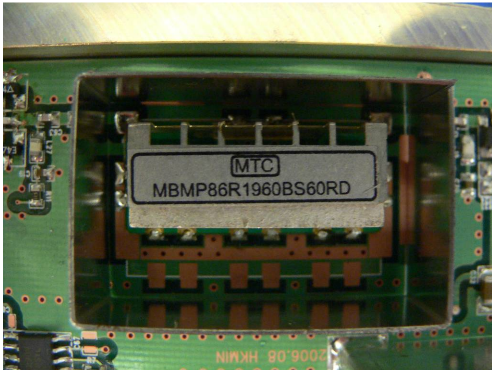
EUT- RF shielding off View 1
