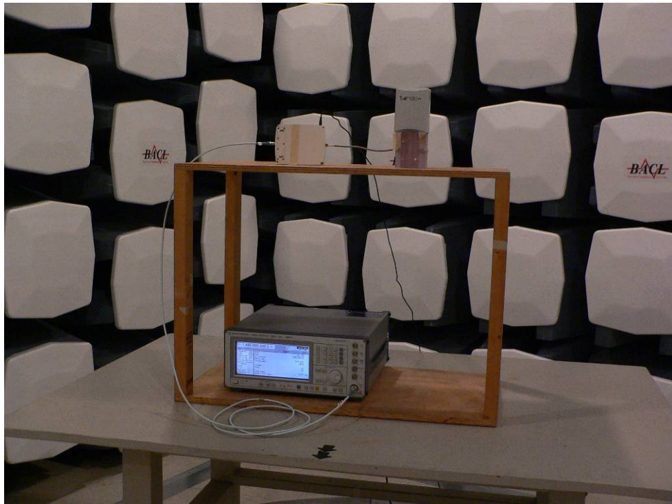
Reverse Radiated Emission – Rear View
