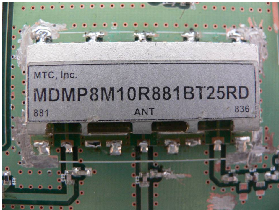
RF shielding off View 4
