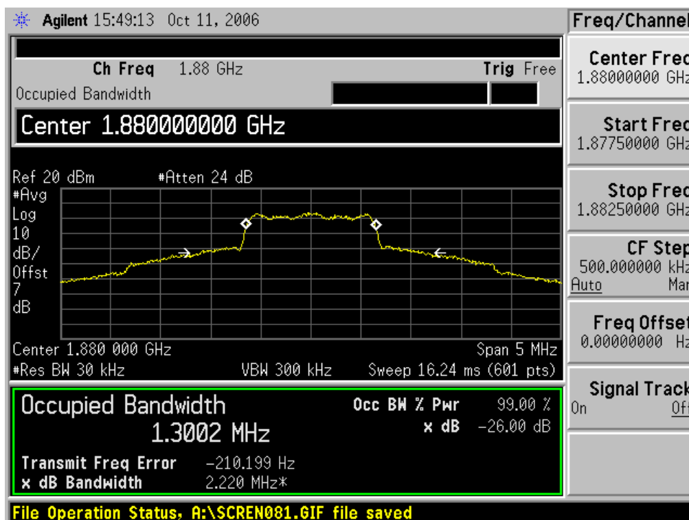
Channel 600
