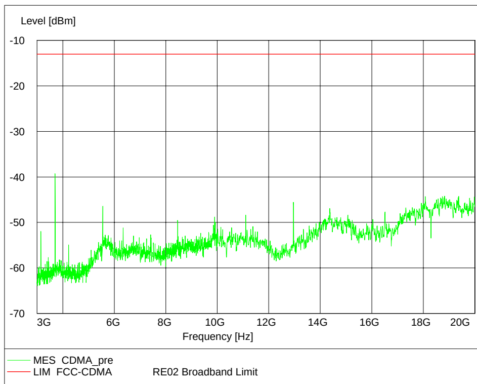
Channel 25, 3GHz~20GHz
