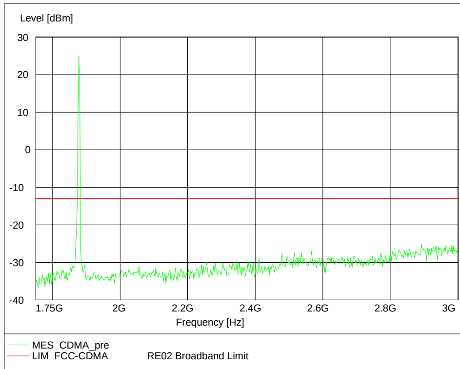
Channel 600, 1750MHz~3GHz
