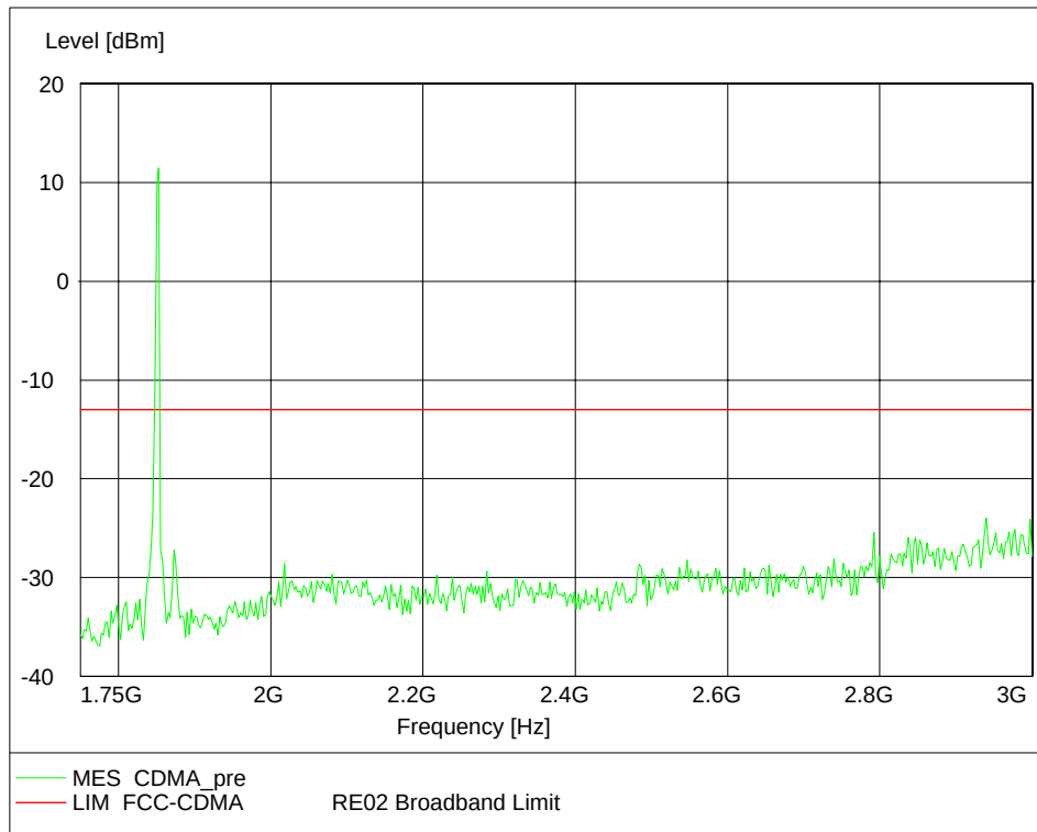
Channel 25, 1750MHz~3GHz
