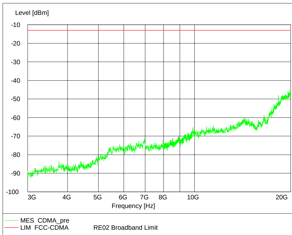
Channel 600, 3GHz~20GHz
