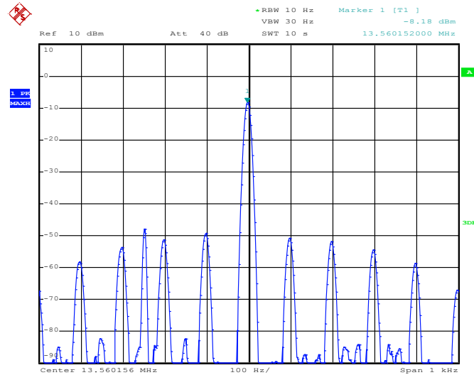
Plot 1: Frequency Error T_{nom} / V_{nom} (example plot)
