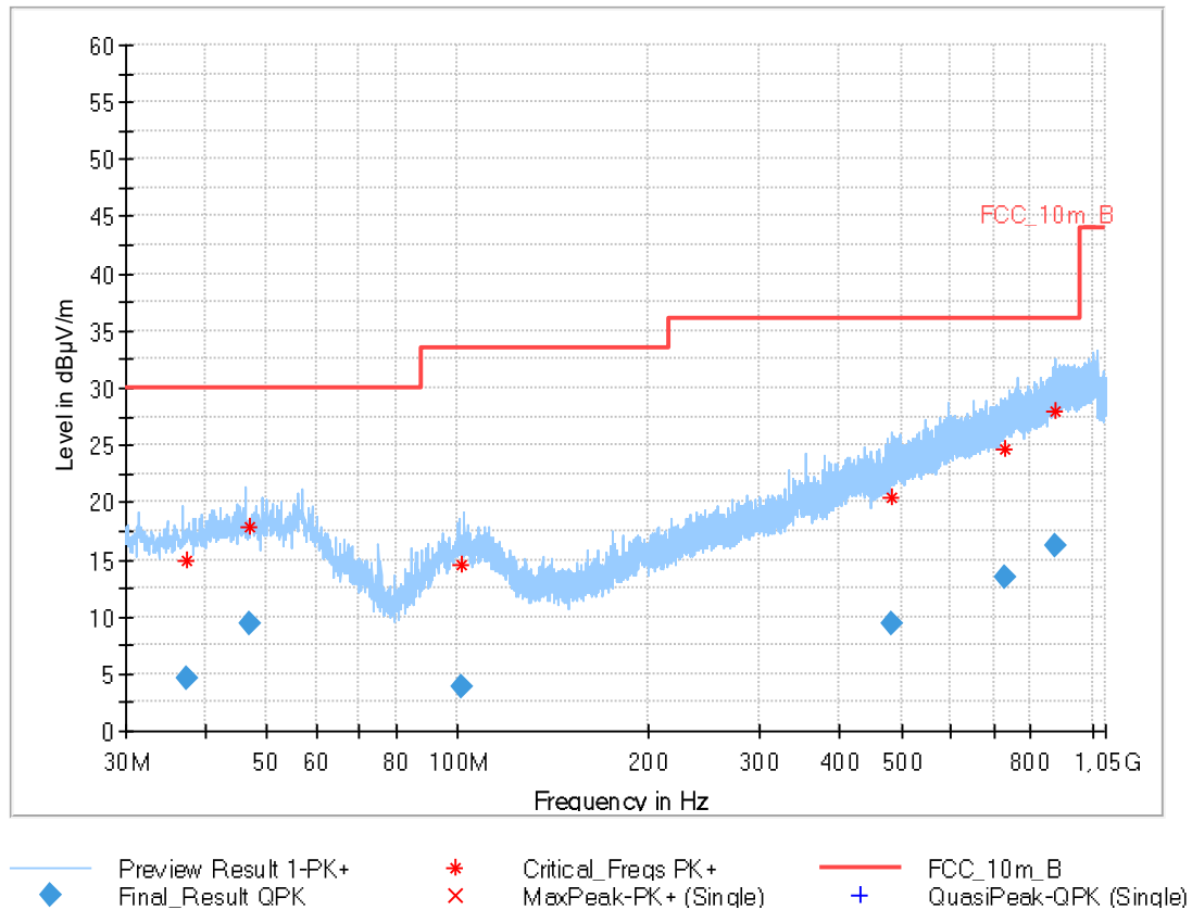
Plot 4: 30 MHz – 1 GHz, vertical and horizontal polarisation
