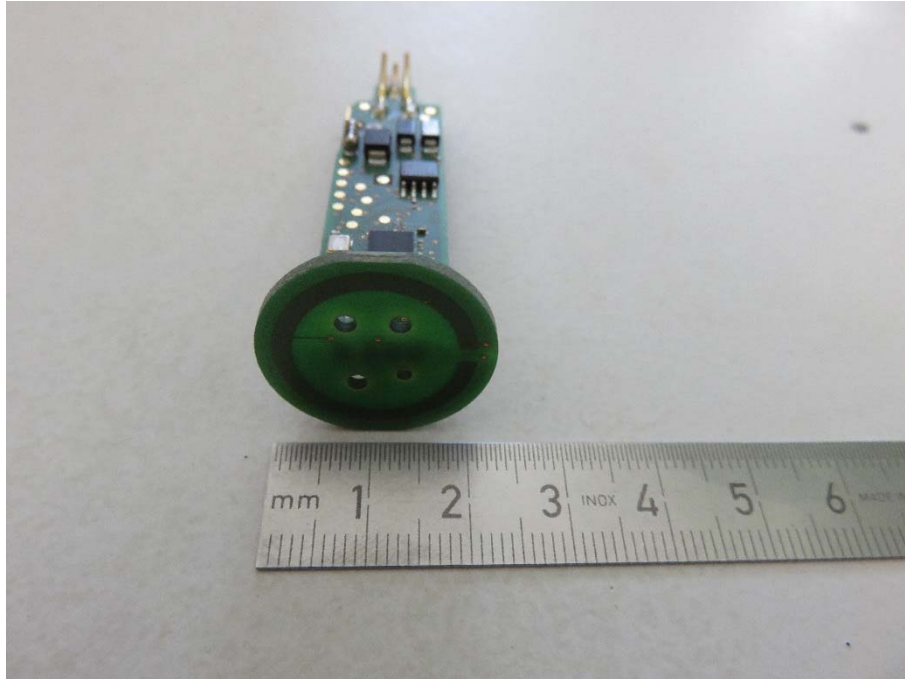
Photo 3: DTM 434&436 antenna
