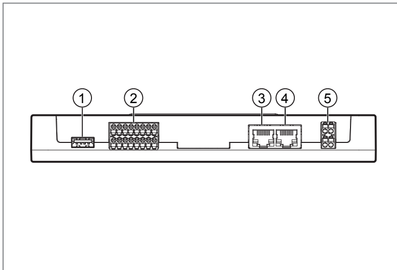
Fig. 4: Bottom-side connectors
