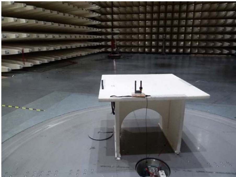
Photo 3: Test setup for radiated measurement from 30MHz to 1GHz
