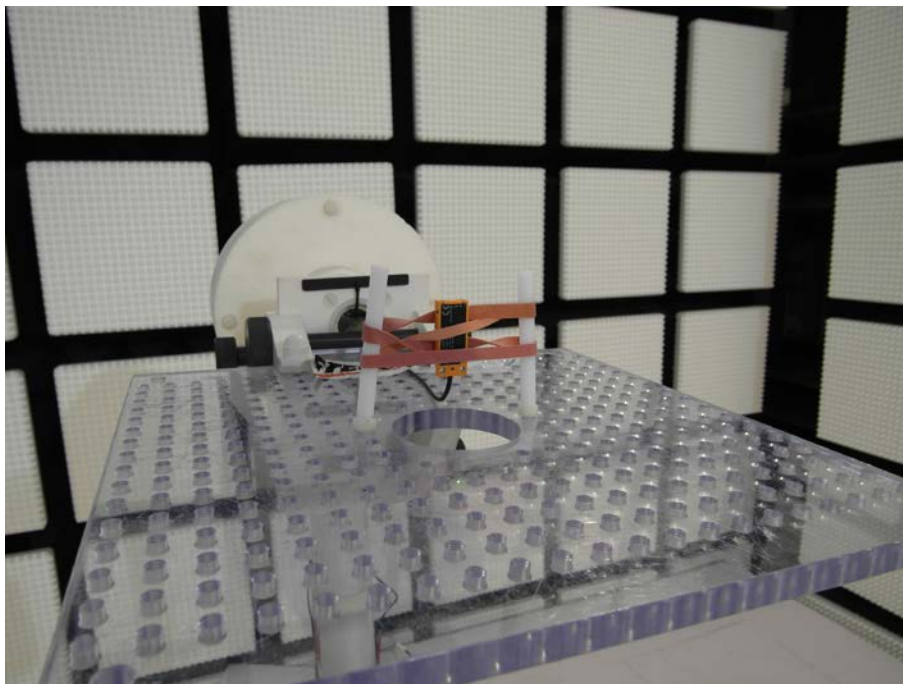
Photo 1: Radiated test setup
