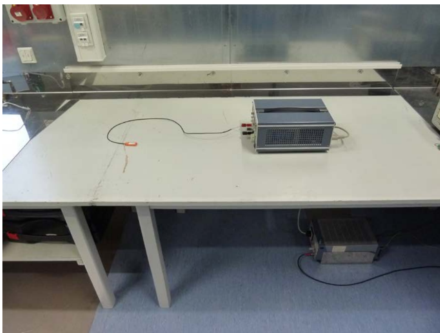
Photo 4: Test setup for conducted measurement on DC line
