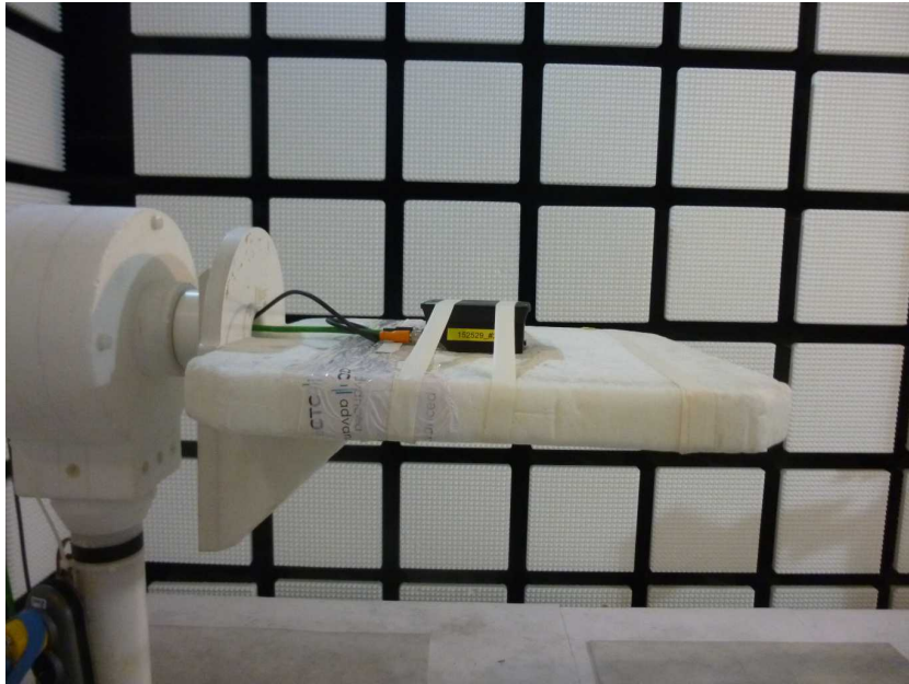
Photo 3: EUT at the anechoic chamber, test setup without tag
