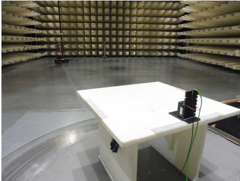
Photo 15: EUT at the semi-anechoic chamber
