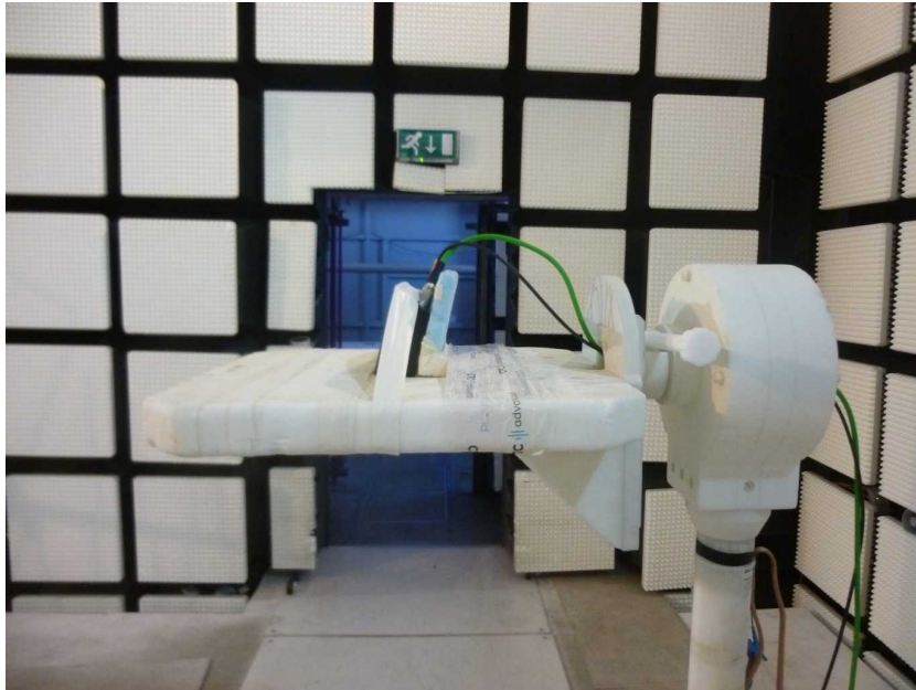
Photo 9: EUT at the anechoic chamber, test setup with tag in 20 cm distance
