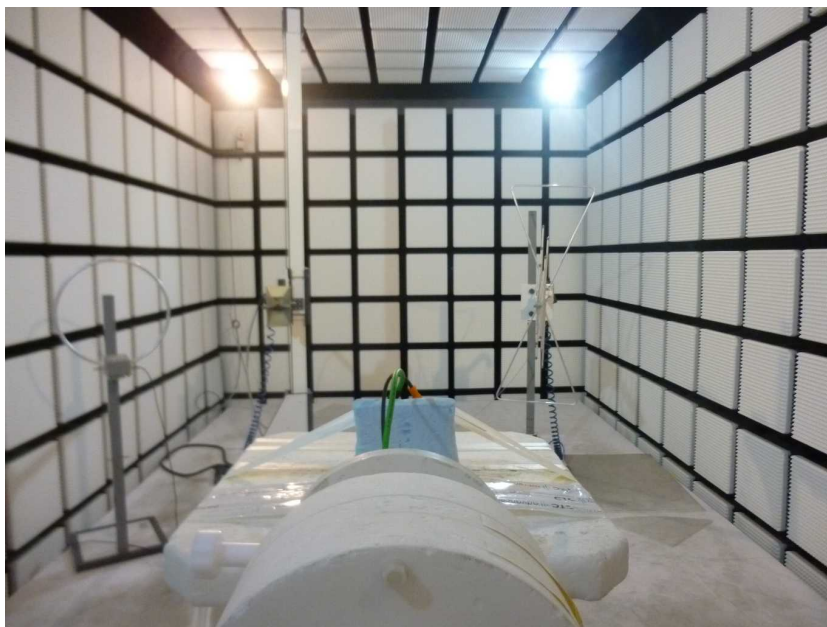
Photo 8: EUT at the anechoic chamber, test setup with tag in 20 cm distance
