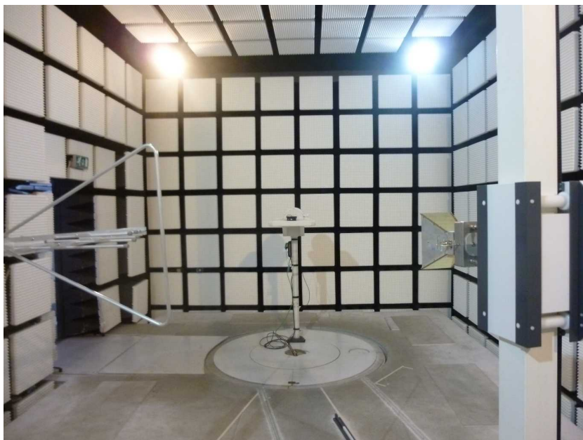
Photo 6: EUT at the anechoic chamber, test setup without tag
