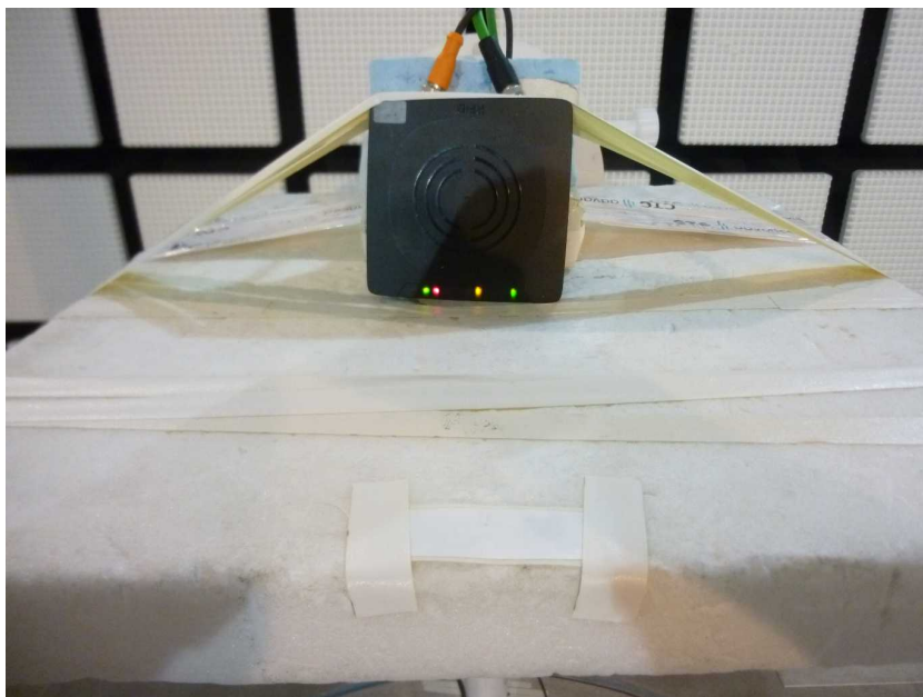
Photo 12: EUT at the anechoic chamber, test setup with tag in 20 cm distance
