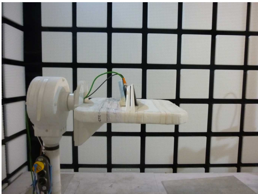
Photo 10: EUT at the anechoic chamber, test setup with tag in 20 cm distance
