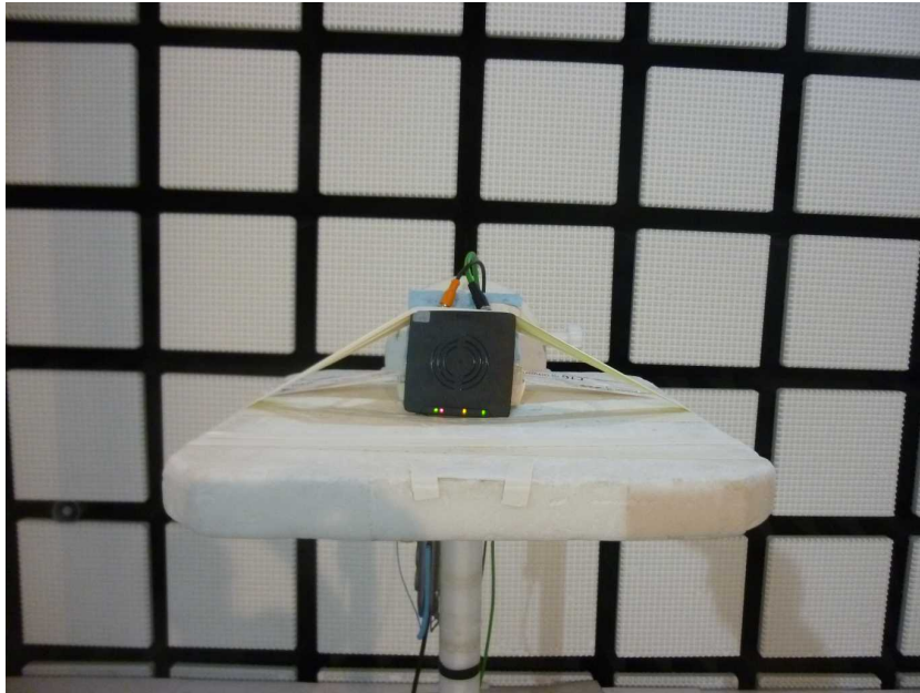
Photo 11: EUT at the anechoic chamber, test setup with tag in 20 cm distance
