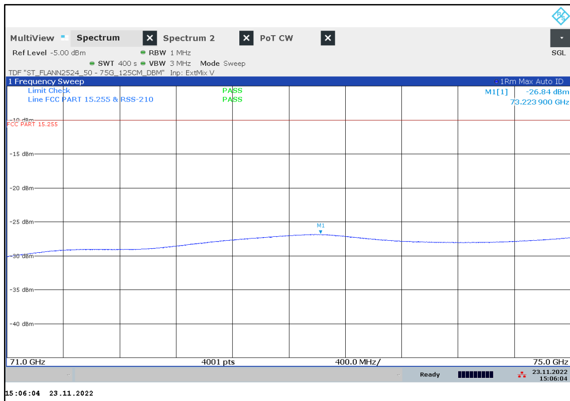
Plot 43: 71 GHz – 75 GHz, CW F_{\text{mid}}
