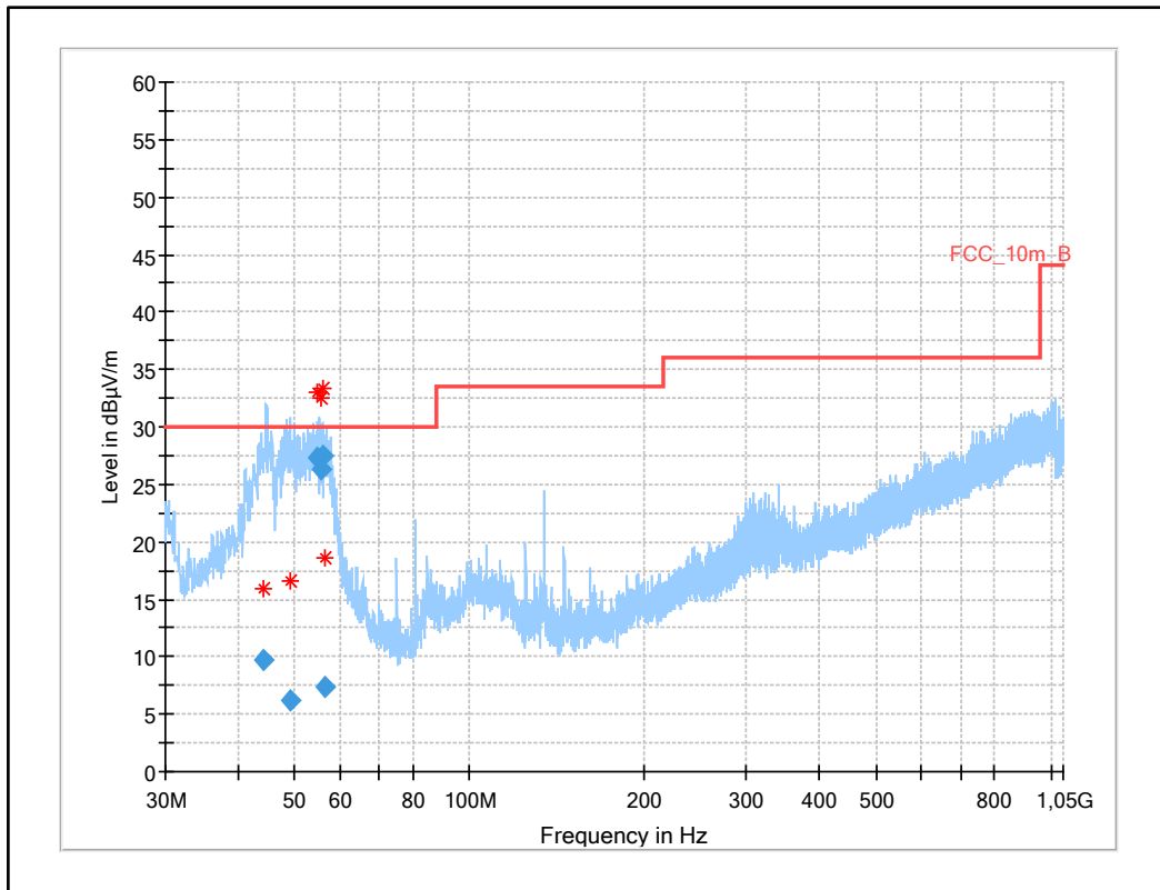
Plot 20: 30 MHz – 1GHz, Mode A
