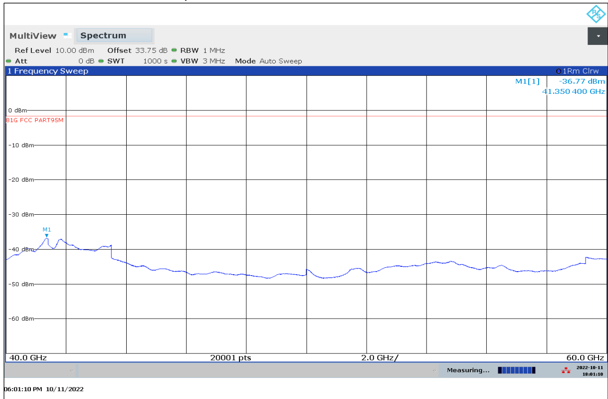
Plot 7: 40 GHz – 60 GHz, valid for specified modes, antenna vertical / horizontal
