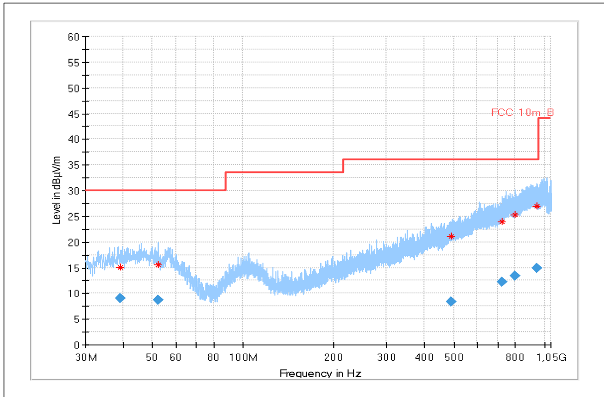
Plot 3: 30 MHz – 1 GHz, Fast Mode, antenna vertical / horizontal
