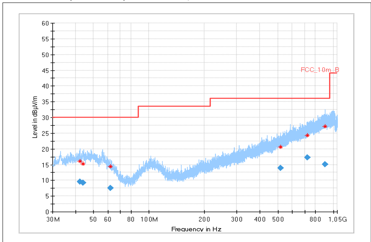
Plot 2: 30 MHz – 1 GHz, Normal Mode, antenna vertical / horizontal
