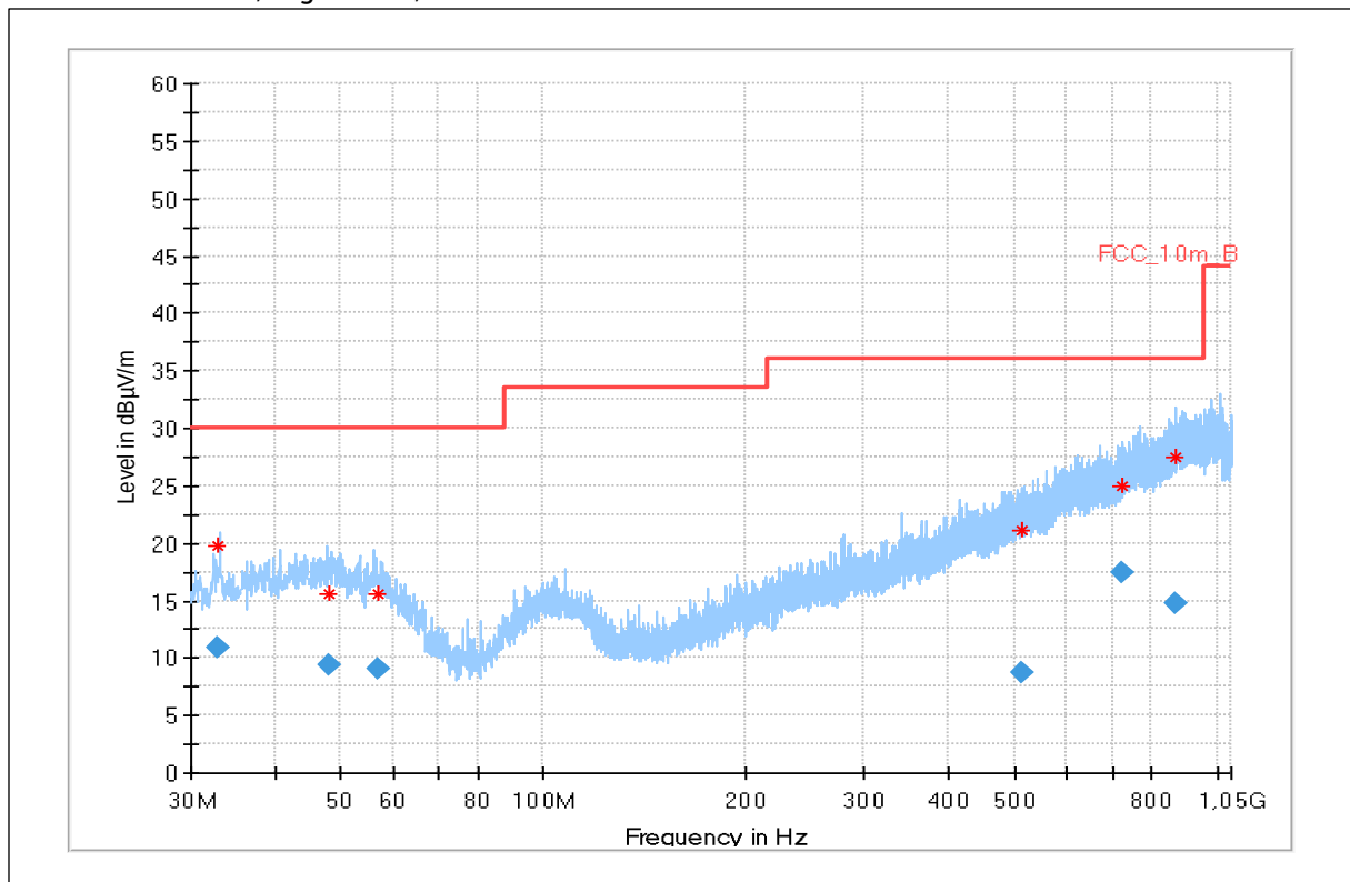
Plot 4: 30 MHz – 1 GHz, High Mode, antenna vertical / horizontal
