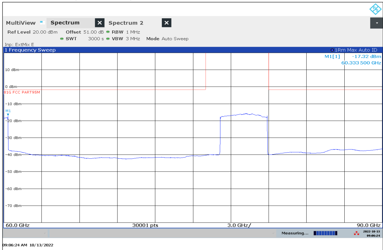
Plot 8: 60 GHz – 90 GHz, Normal mode, antenna vertical / horizontal
