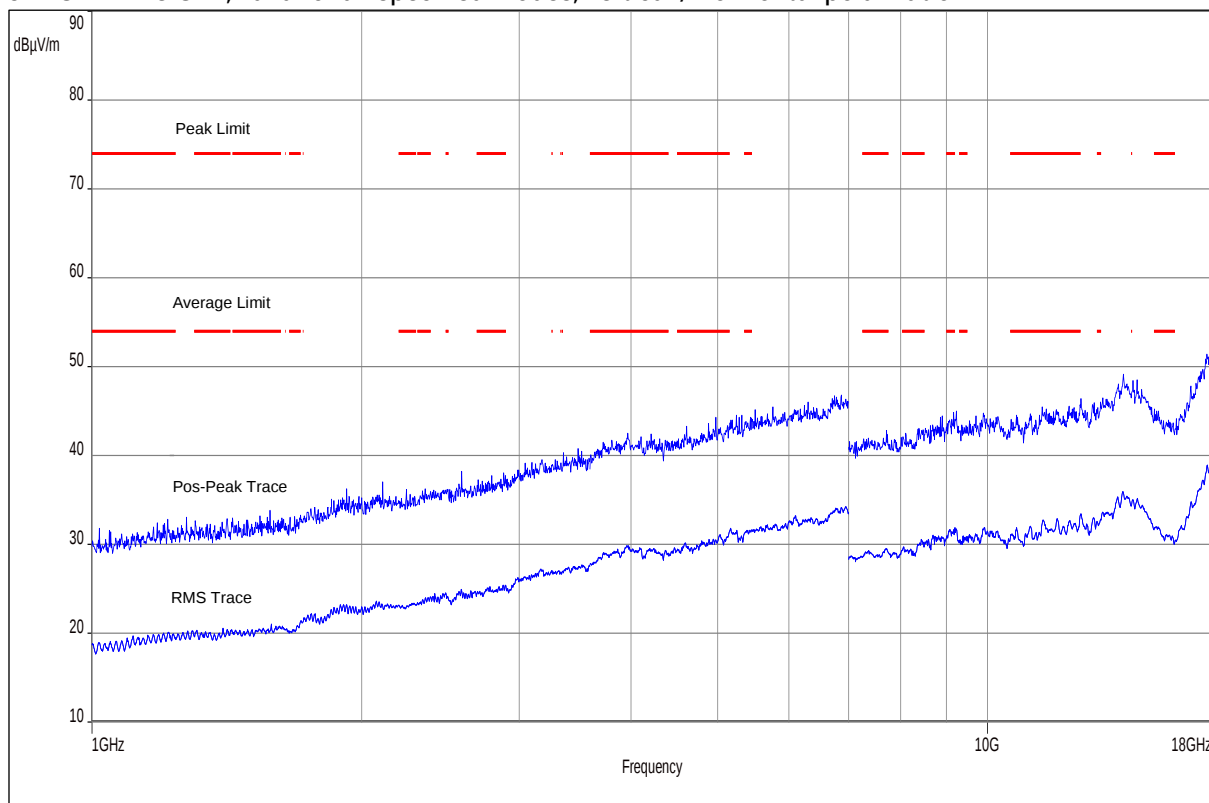
Plot 5: 1 GHz – 18 GHz, valid for all specified modes, vertical / horizontal polarization
