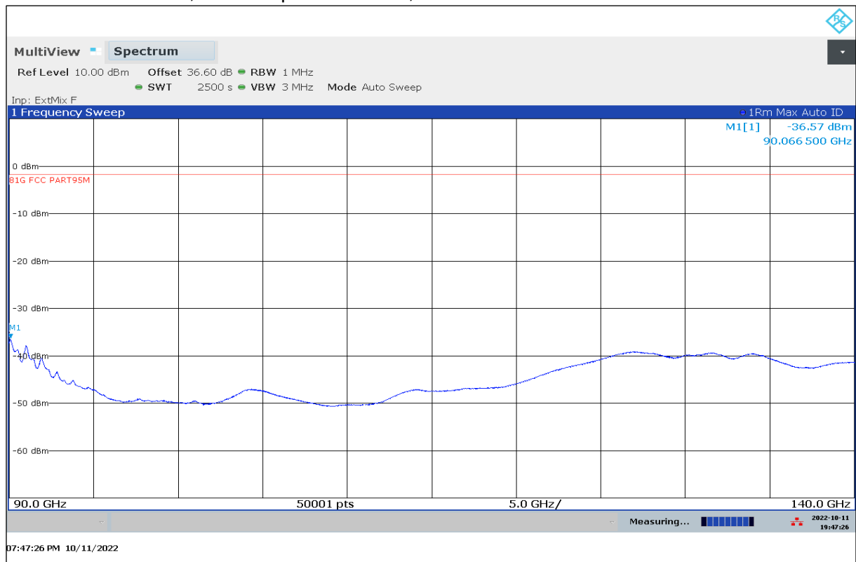
Plot 11: 90 GHz – 140 GHz, valid for specified modes, antenna vertical / horizontal
