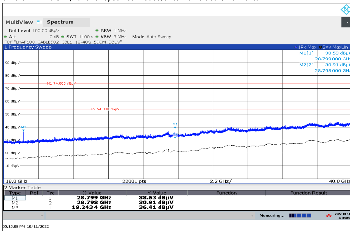
Plot 6: 18 GHz – 40 GHz, valid for specified modes, antenna vertical / horizontal
