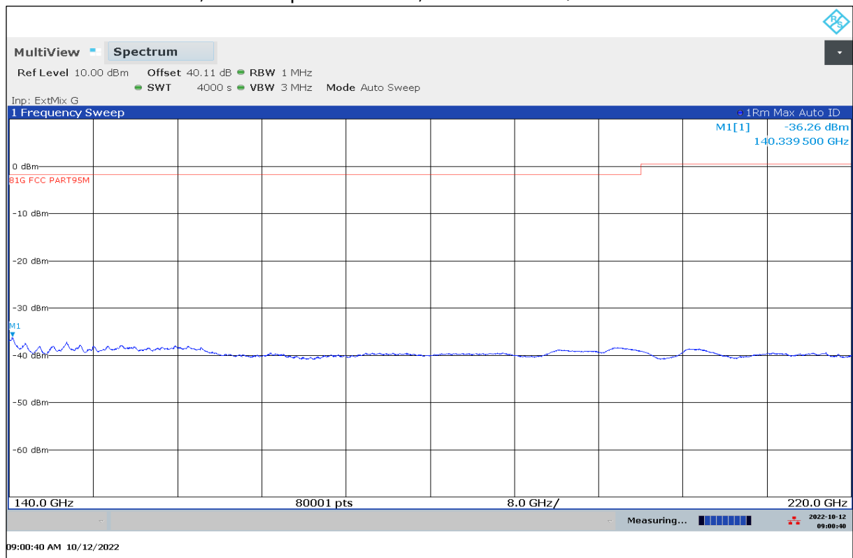
Plot 12: 140 GHz – 220 GHz, valid for specified modes, antenna vertical / horizontal
