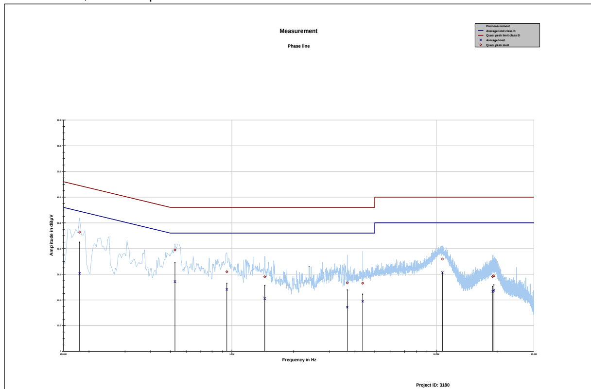
Plot 14: Phase line, Valid for specified modes
