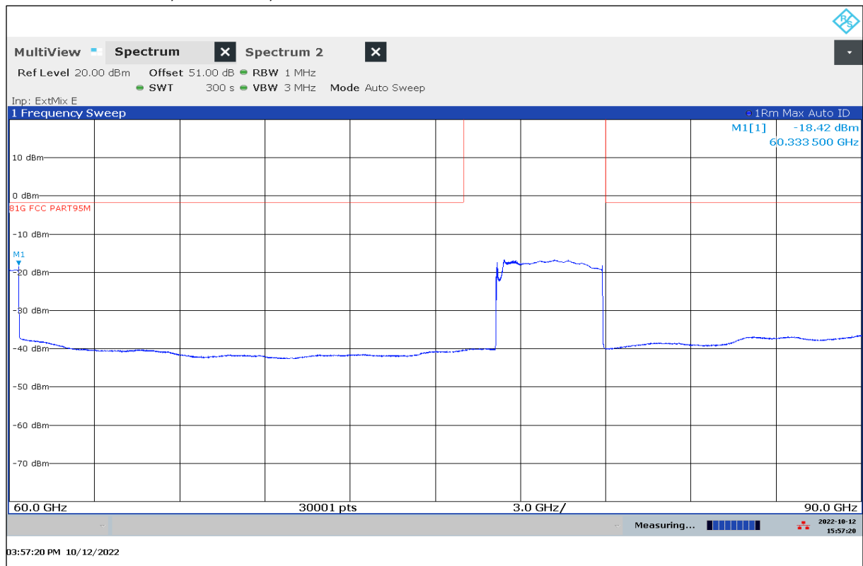
Plot 9: 60 GHz – 90 GHz, Fast mode, antenna vertical / horizontal
