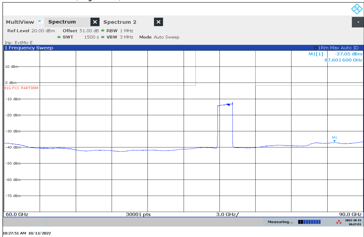
Plot 10: 60 GHz – 90 GHz, High mode, antenna vertical / horizontal
