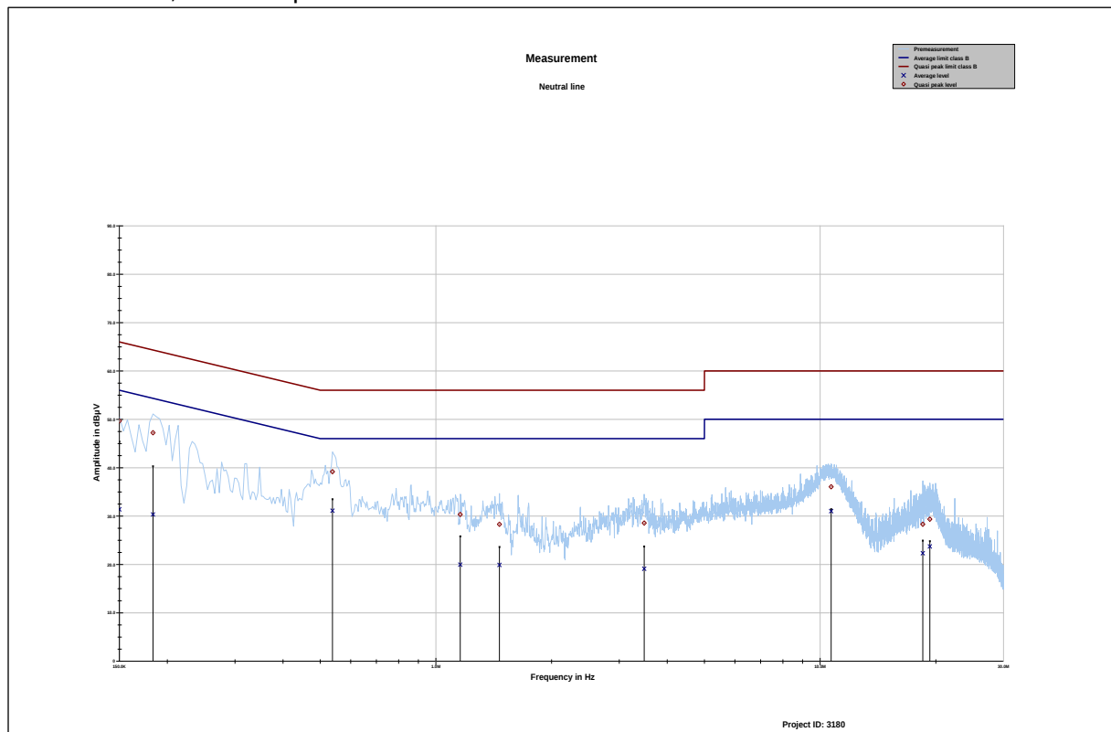
Plot 15: Neutral line, Valid for specified modes
