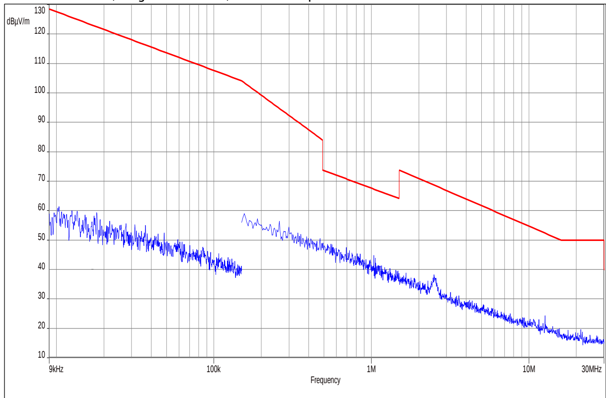
Plot 1: 9 kHz – 30 MHz, Magnetic antenna, valid for all specified modes
