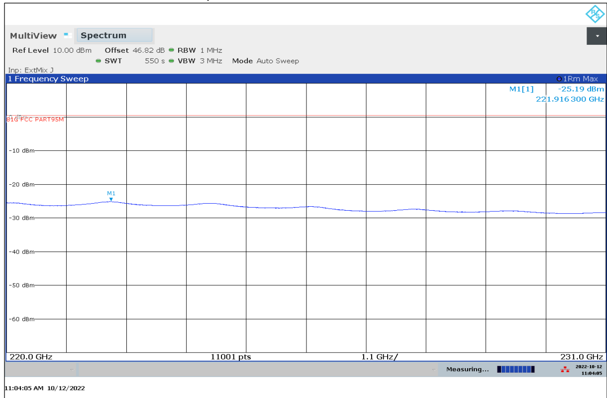
Plot 13: 220 GHz – 231 GHz, valid for specified modes, antenna vertical / horizontal
