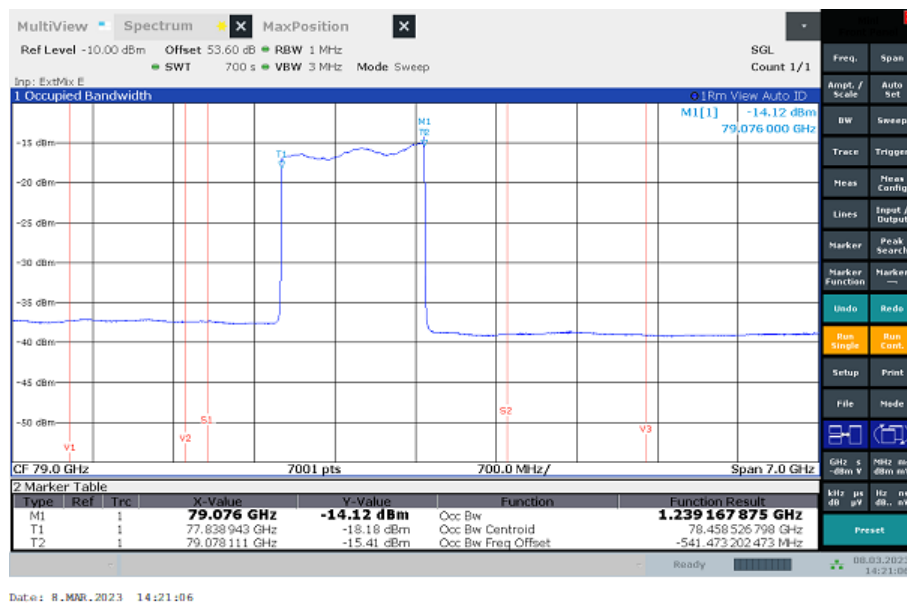
Systems EN # Bandwidth 99pct ~ Mode: High 77000-81000 MHz 99PCT
