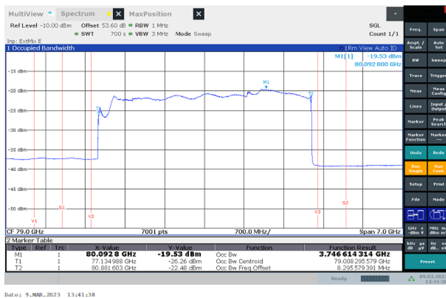
Systems EN # Bandwidth 99pct ~ Mode: Fast 77000-81000 MHz 99PCT
