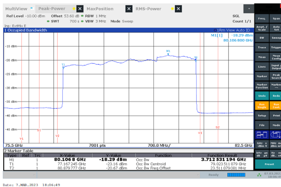
Systems EN # Bandwidth 99pct ~ Mode: Normal 77000-81000 MHz 99PCT
