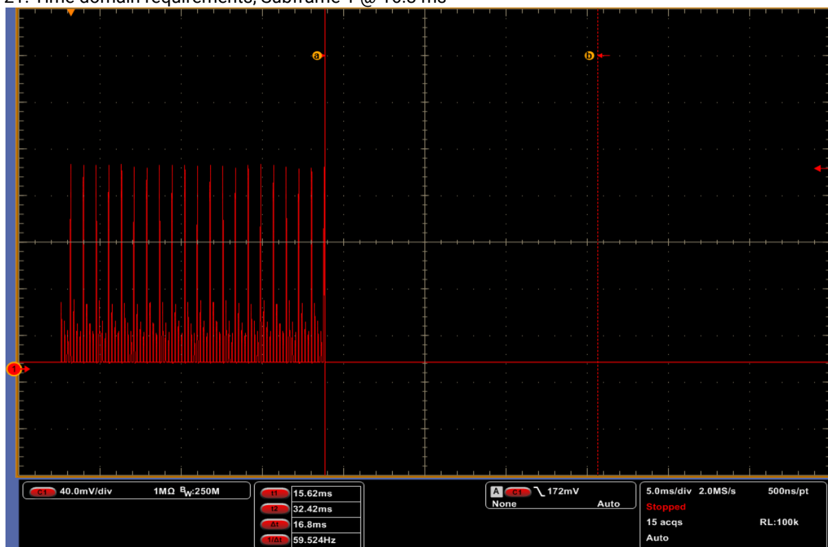
Plot 21: Time domain requirements, Subframe 1 @ 16.8 ms
