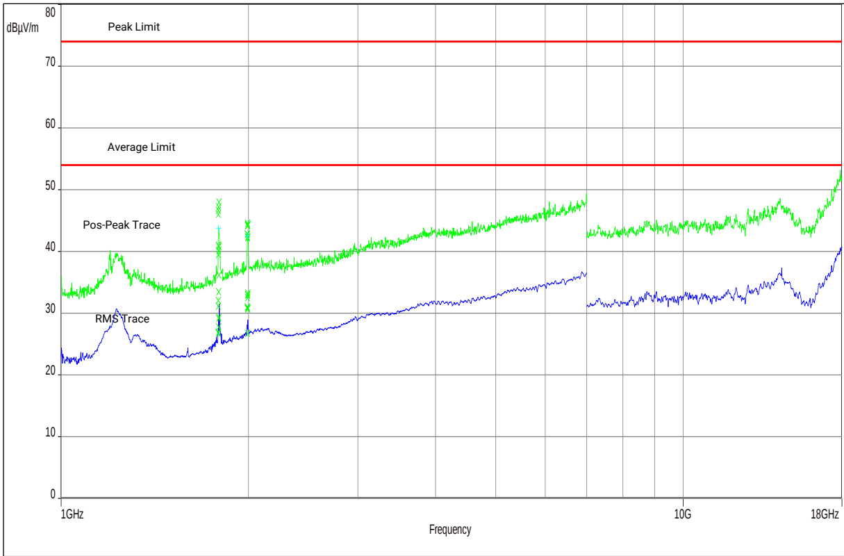
Plot 24: 1 GHz – 18 GHz, antenna vertical / horizontal
