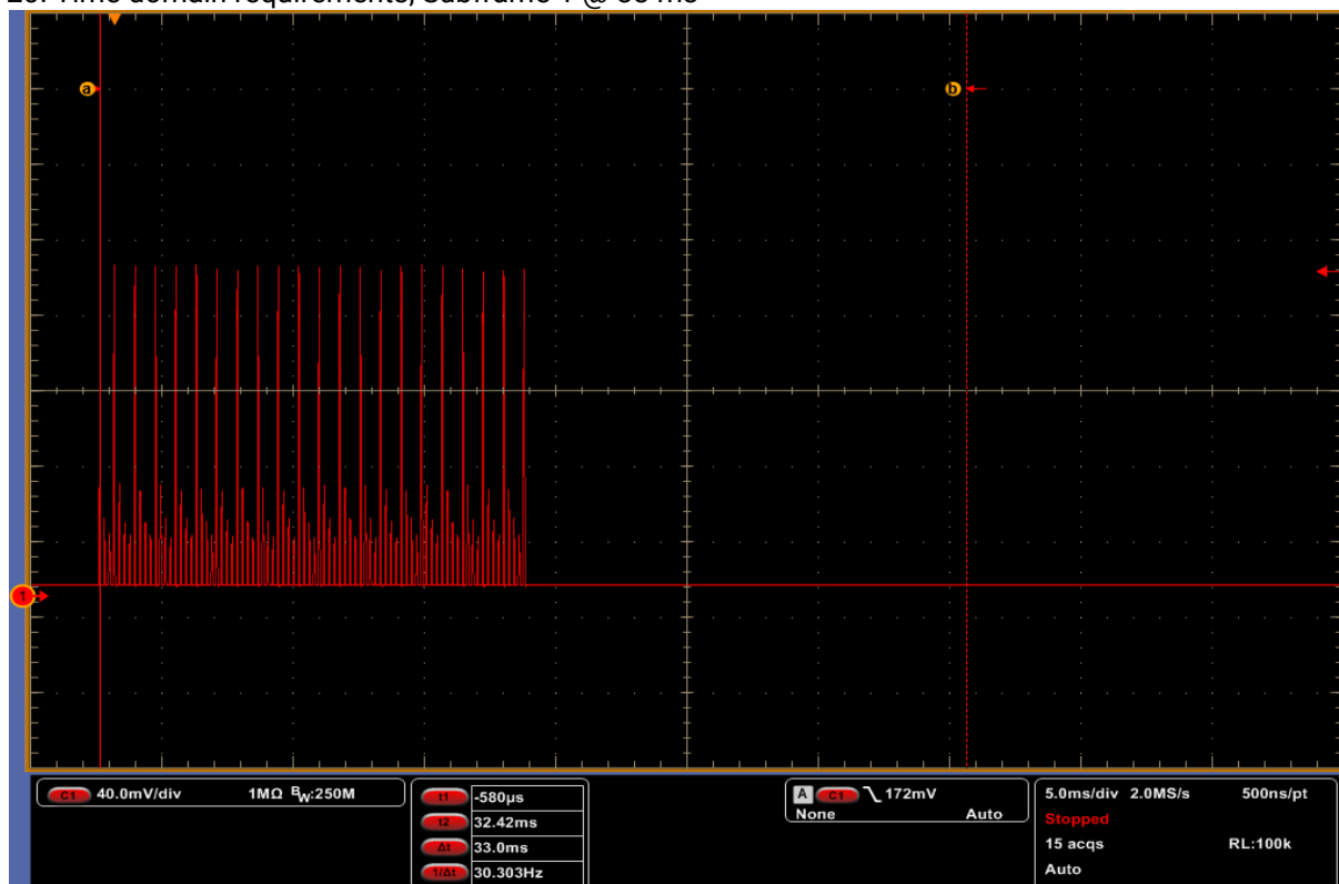
Plot 20: Time domain requirements, Subframe 1 @ 33 ms
