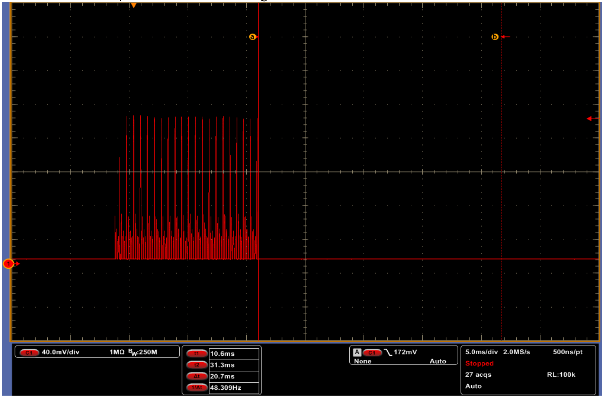
Plot 19: Time domain requirements, Subframe 0 @ 20.7ms
