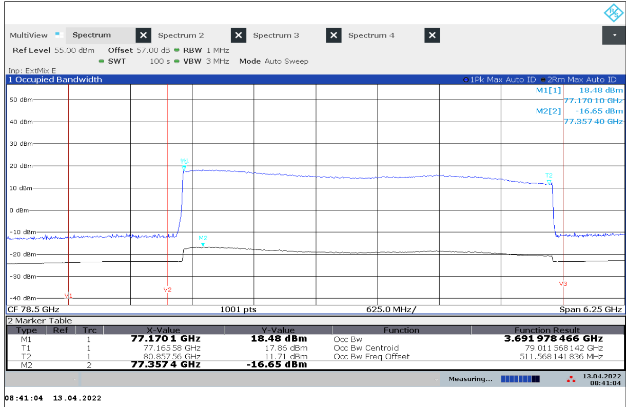
Plot 25: Normal Mode, OBW, -20 °C / V min-max
