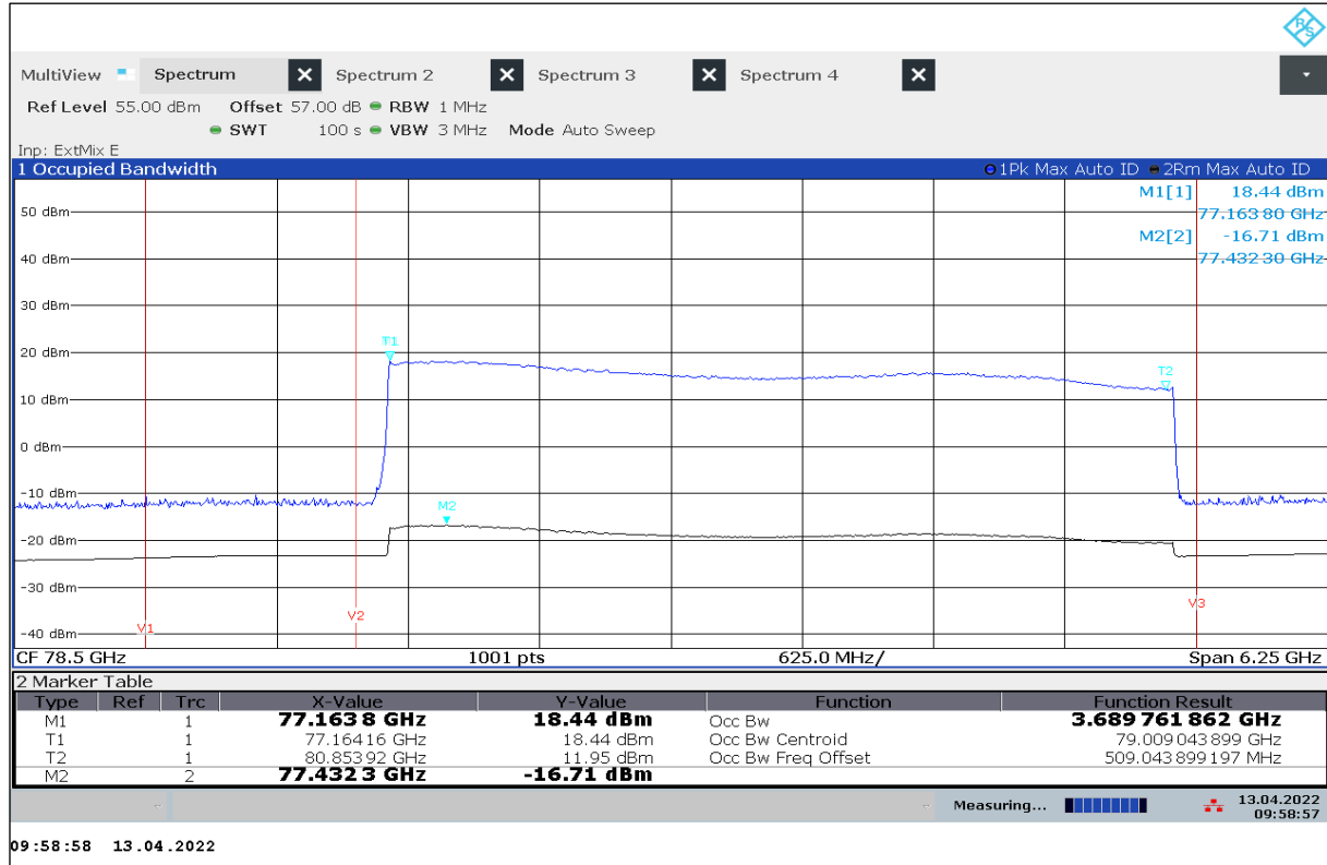
Plot 27: Normal Mode, OBW, 0 °C / V min-max
