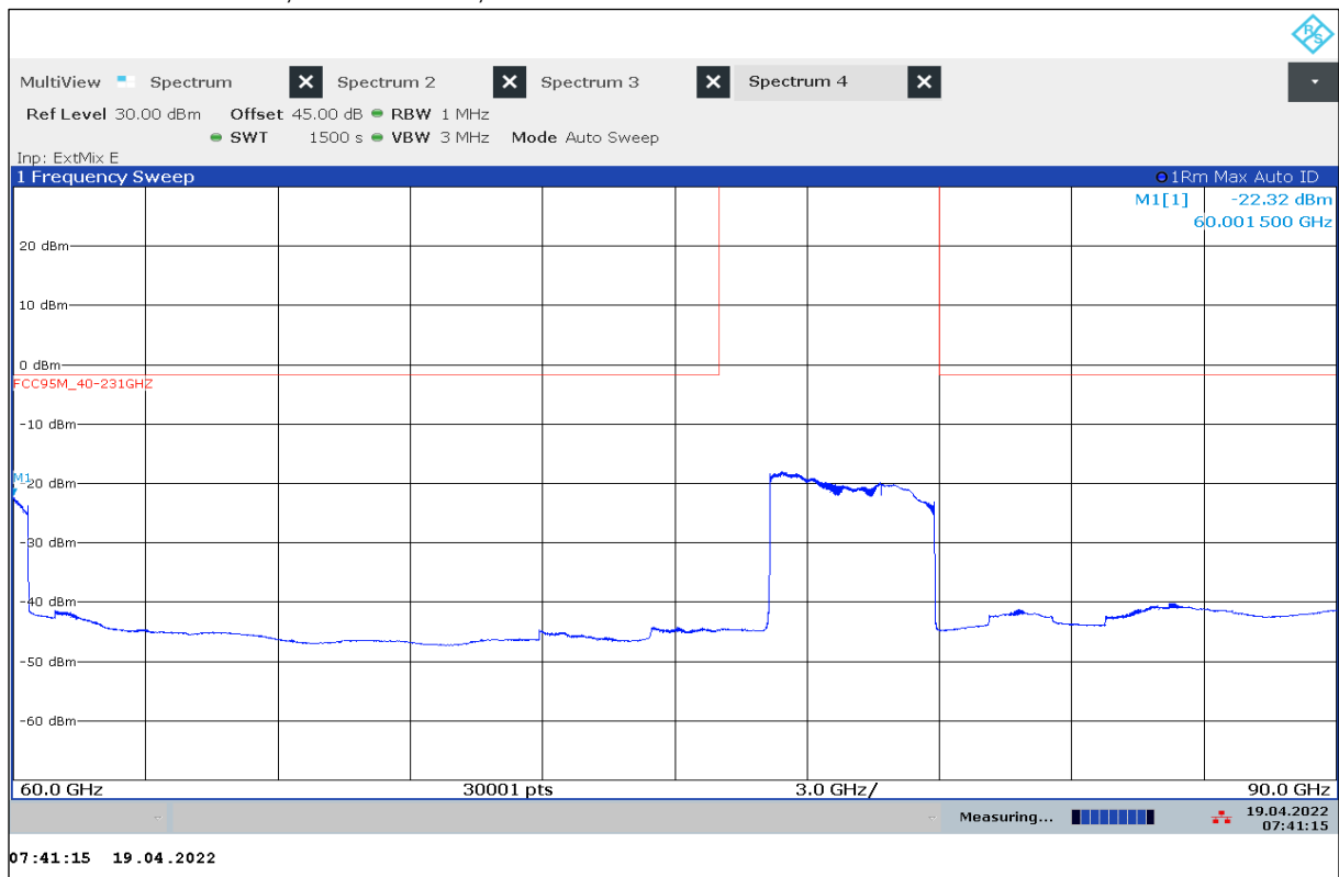
Plot 14: 60 GHz – 90 GHz, Normal Mode, antenna vertical / horizontal
