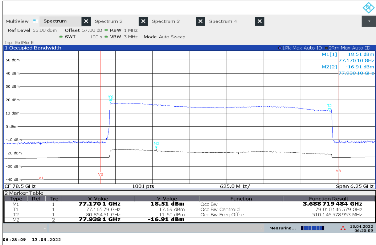
Plot 1: OBW, EIRP Peak Power, Normal Mode, T_{nom} / V_{min-max}
