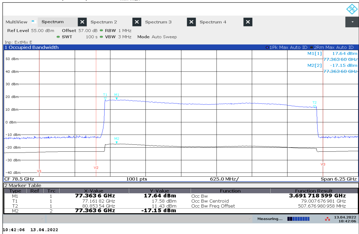
Plot 32: Normal Mode, OBW, 50 °C / V min-max
