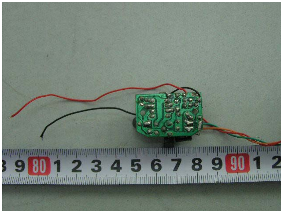
EUT-Charge PCB View (2)
