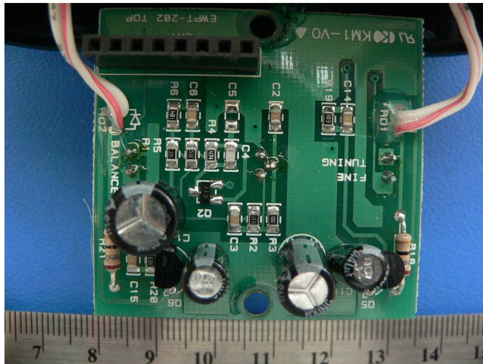
EUT – Board 2 Component side view
