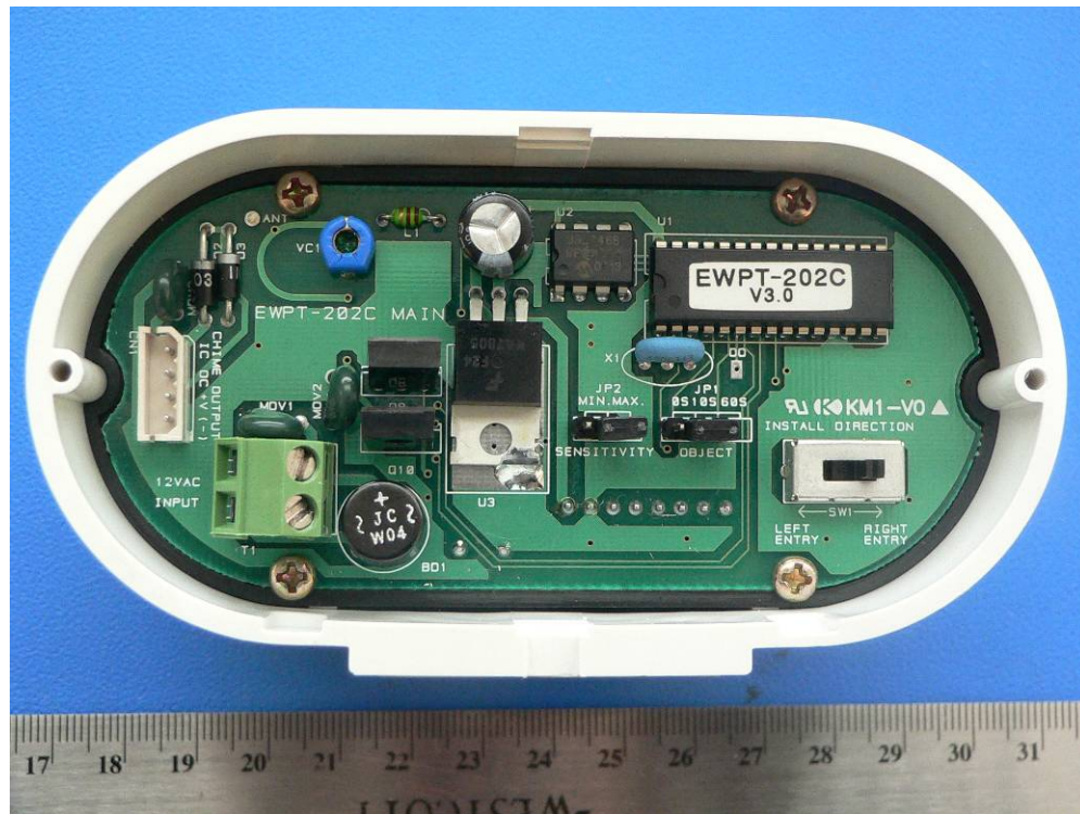
EUT – Chassis off view
