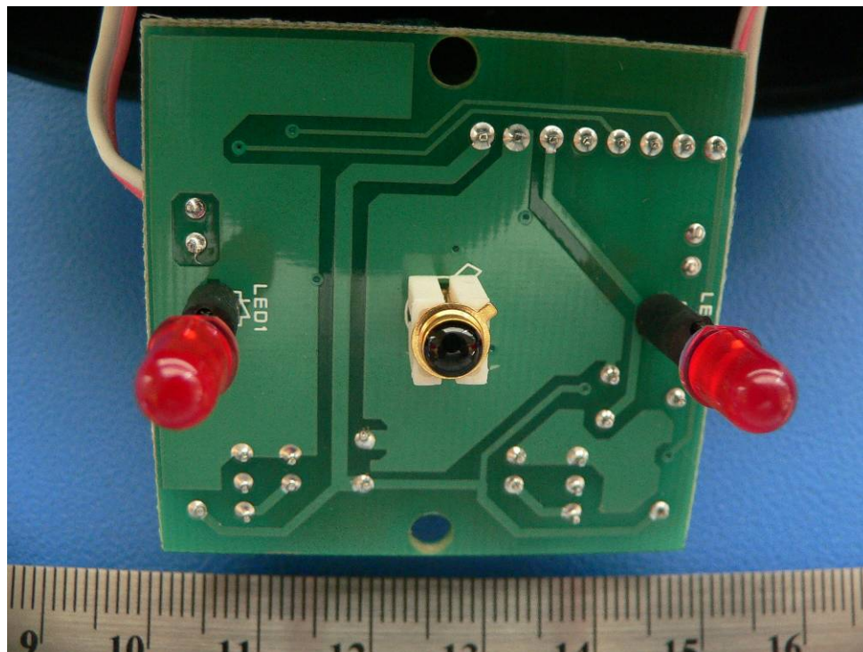
EUT – Board 2 Solder side view
