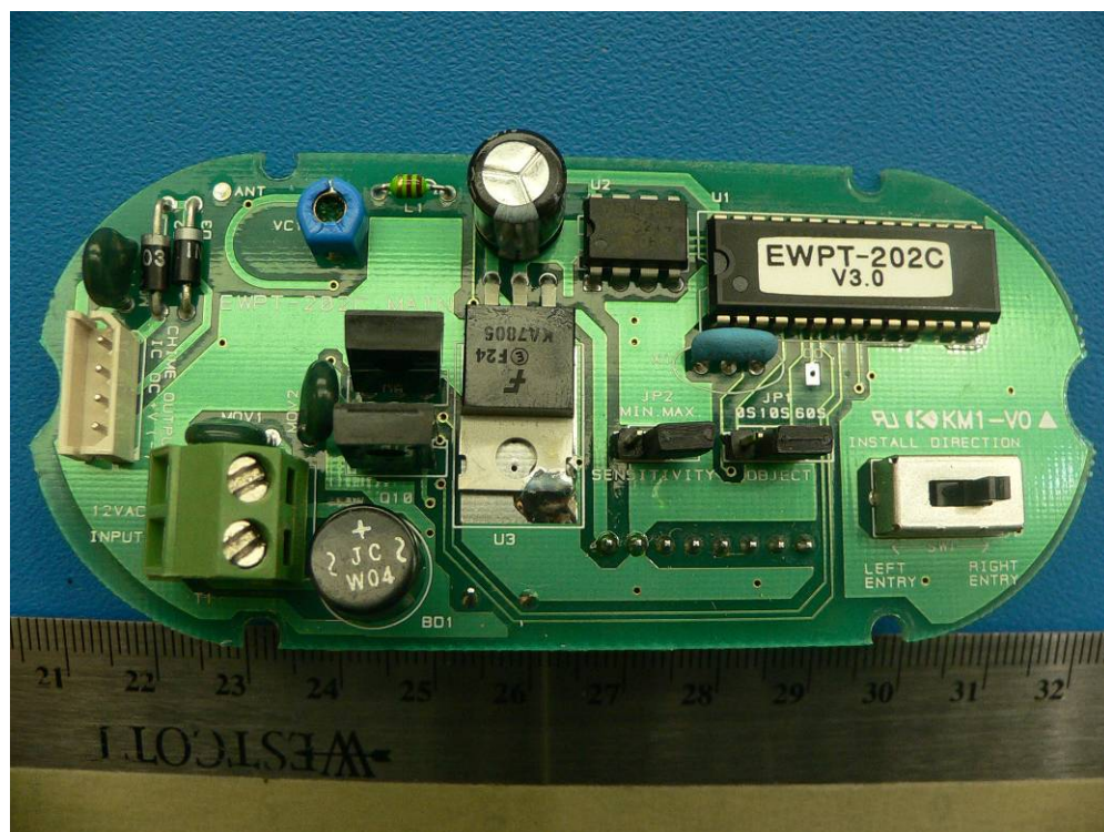
EUT – Board 1 Component side view
