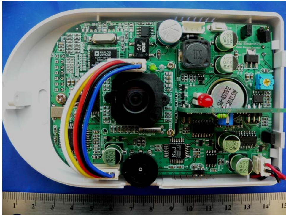
EUT Radio Card- Component view
