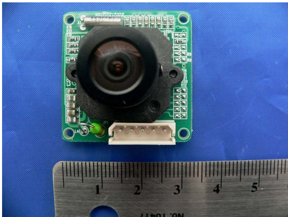
EUT PCB with Camera- Component view
