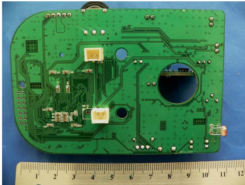
EUT Radio Card- Solder view
