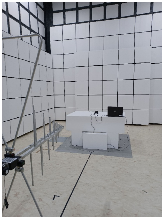
Radiated Test
