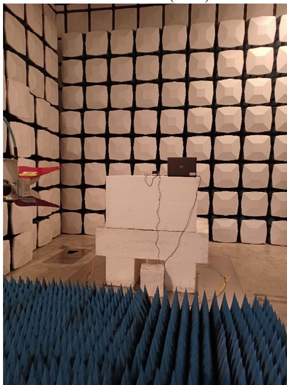
Radiated Test (Horn)
