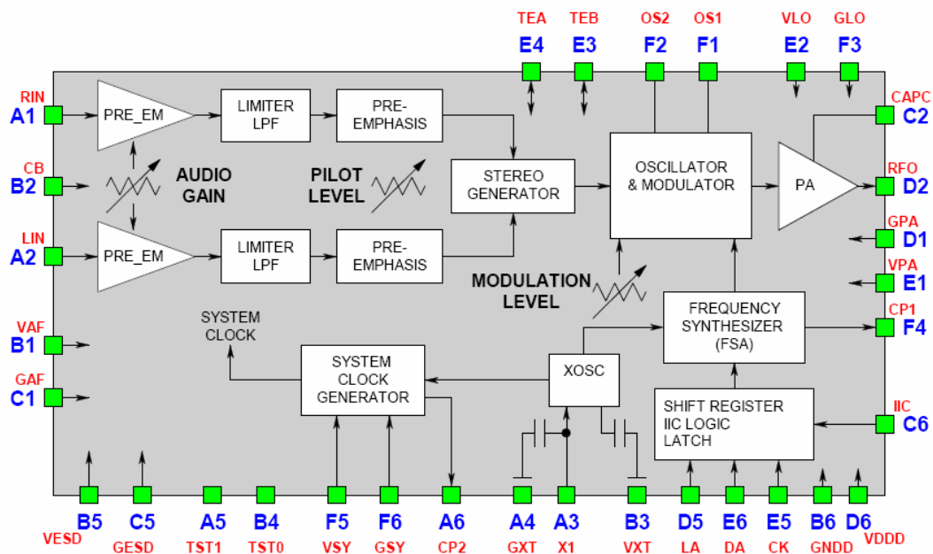
Block Diagram of NS73
