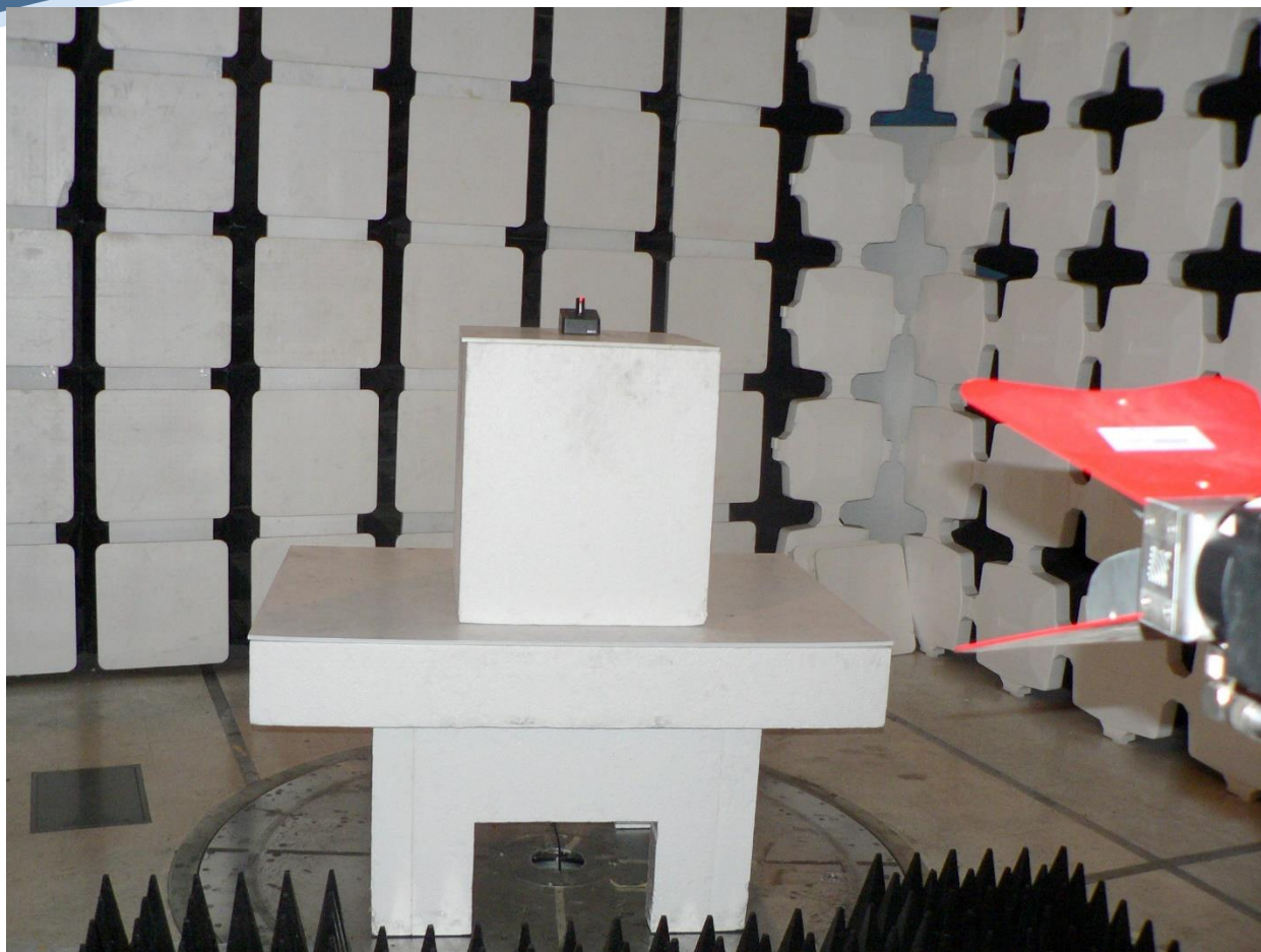
Tx Spurious Above 1GHz
