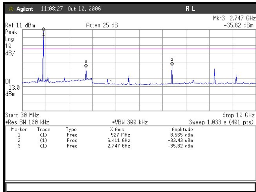
Mid Channel Conducted Emissions 30MHz – 10GHz
