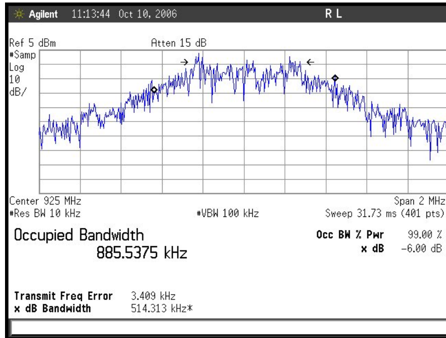
High Ch Occupied Band Width
