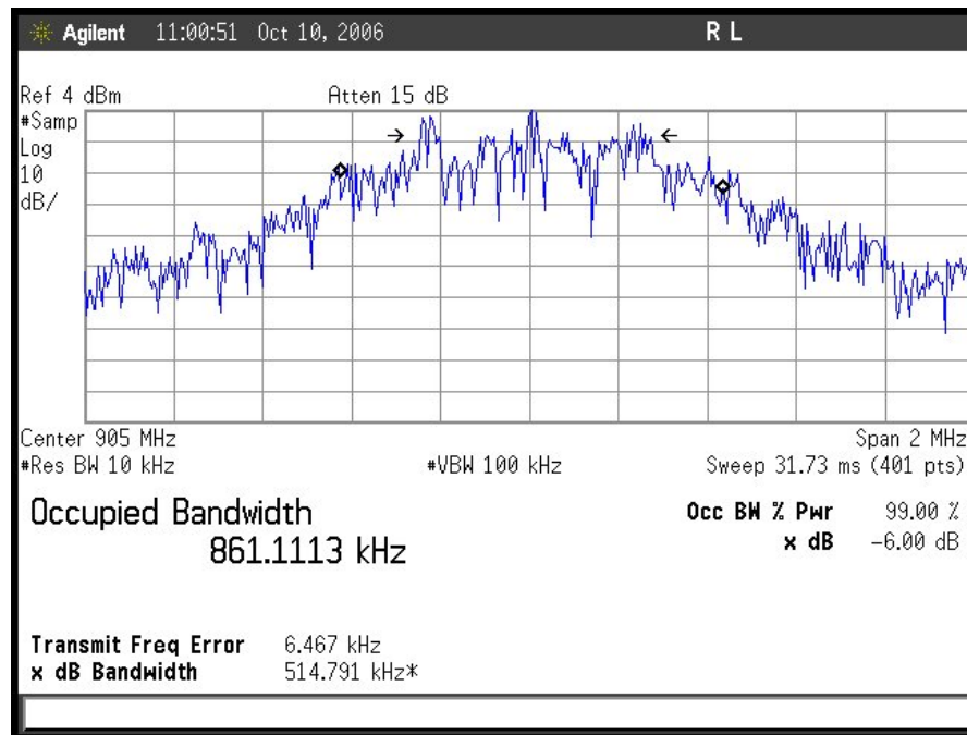
Low Ch Occupied Band Width.
