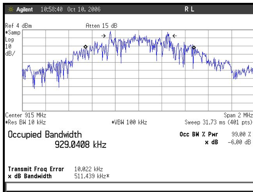
Mid Ch Occupied Band Width
