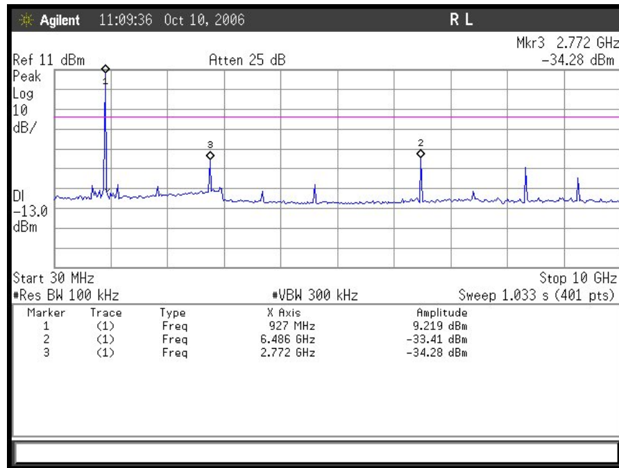
High Channel Conducted Emissions 30MHz- 10GHz
