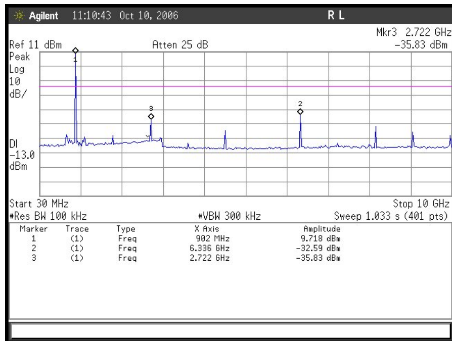
Low Channel Conducted Emissions 30MHz - 10GHz
