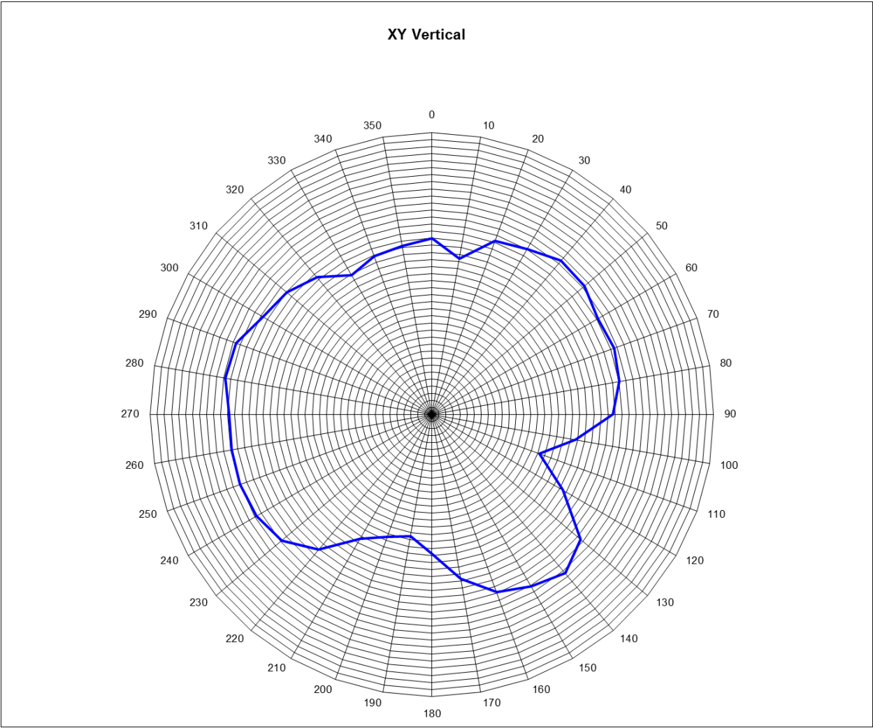
Figure 6 1.5dBi Ref 2400-2485MHz sweep
