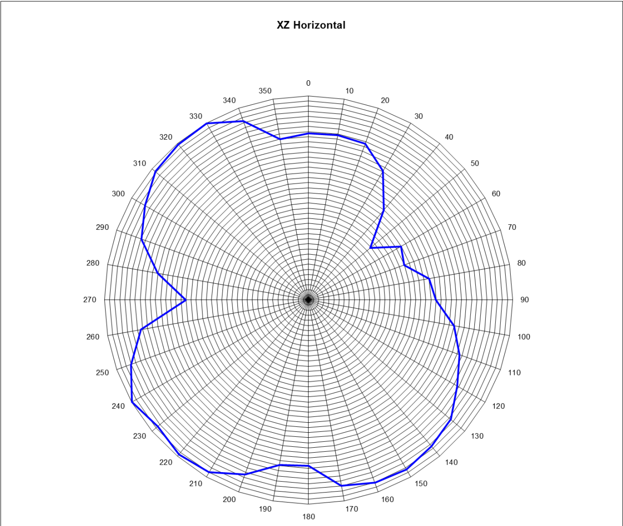
Figure 1 1.5dBi Ref 2400-2485MHz sweep
