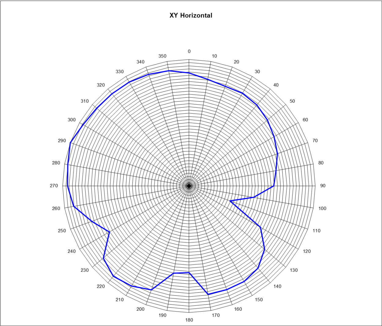
Figure 5 1.5dBi Ref 2400-2485MHz sweep
