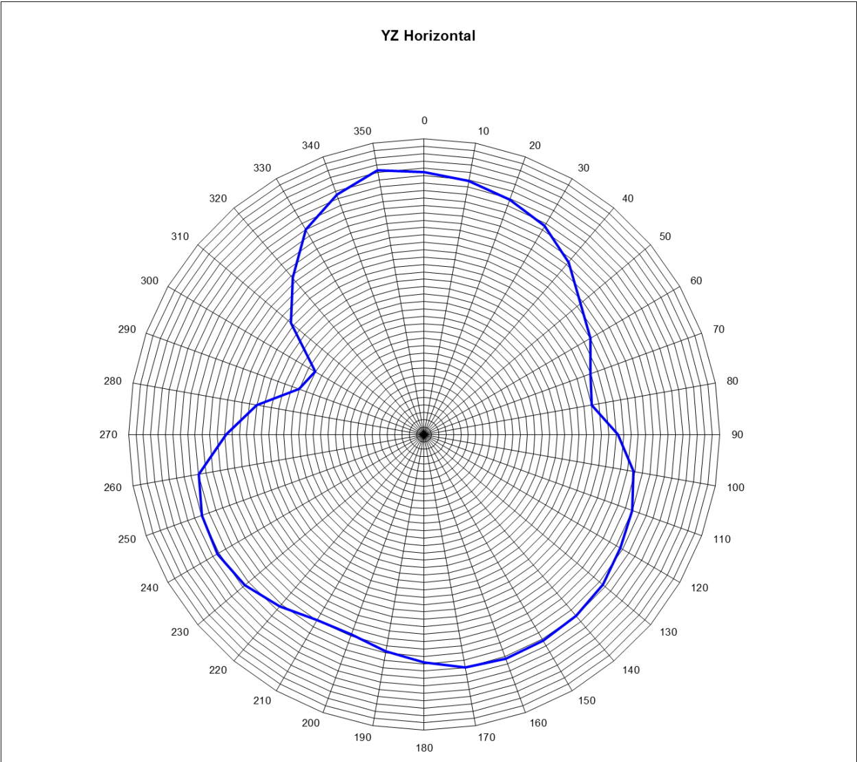
Figure 4 1.5dBi Ref 2400-2485MHz sweep
