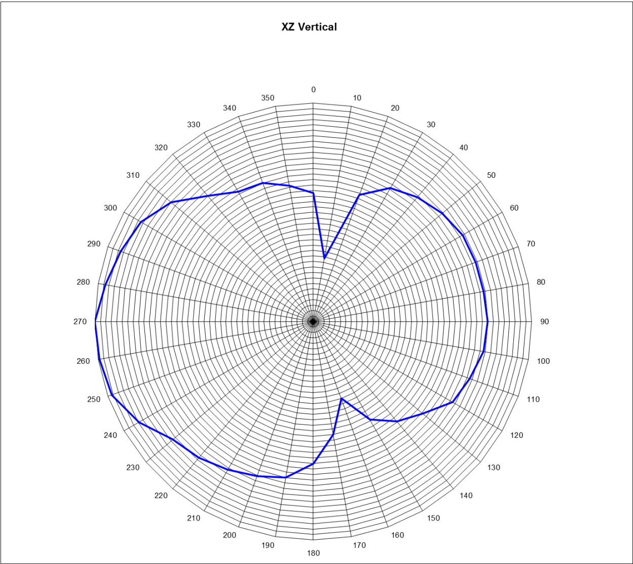
Figure 2 1.5dBi Ref 2400-2485MHz sweep
