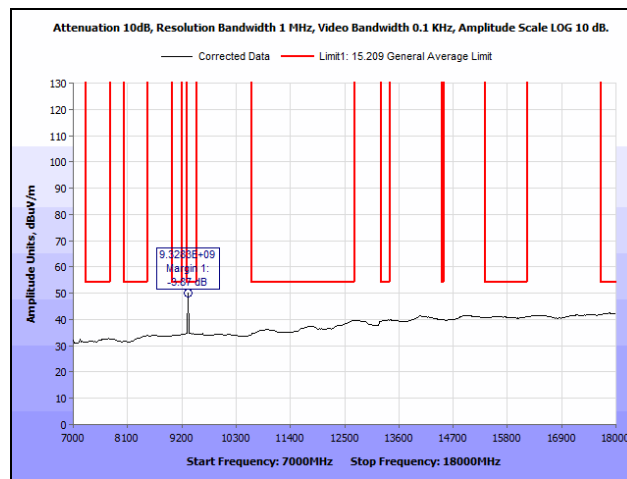
Plot 20. Radiated Spurious Emissions, High Channel, 7 GHz – 18 GHz, Average
