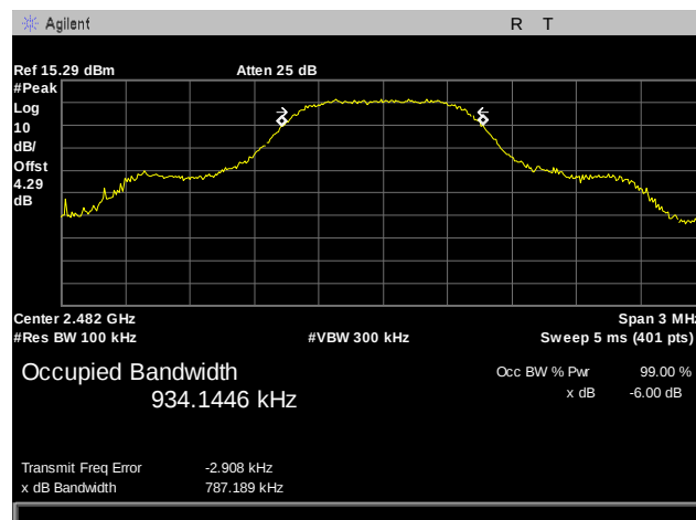
Plot 3. Occupied Bandwidth, High Channel
