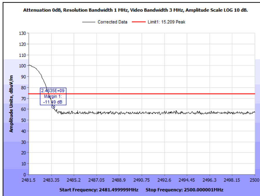
Plot 25. Radiated Restricted Band Edge, High Channel, Peak
