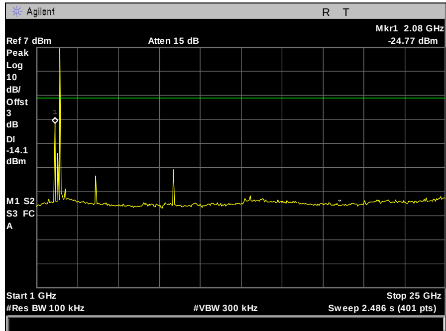
Plot 27. Conducted Spurious Emissions, Low Channel, 1 GHz – 25 GHz
