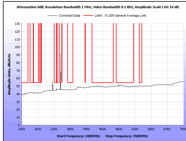
Plot 13. Radiated Spurious Emissions, Mid Channel, 1 GHz – 7 GHz, Average
