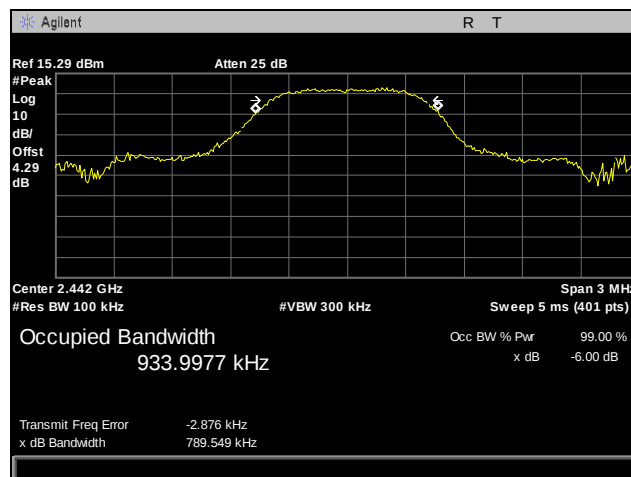
Plot 2. Occupied Bandwidth, Mid Channel
