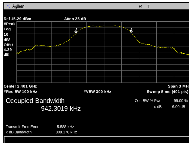
Plot 1. Occupied Bandwidth, Low Channel
