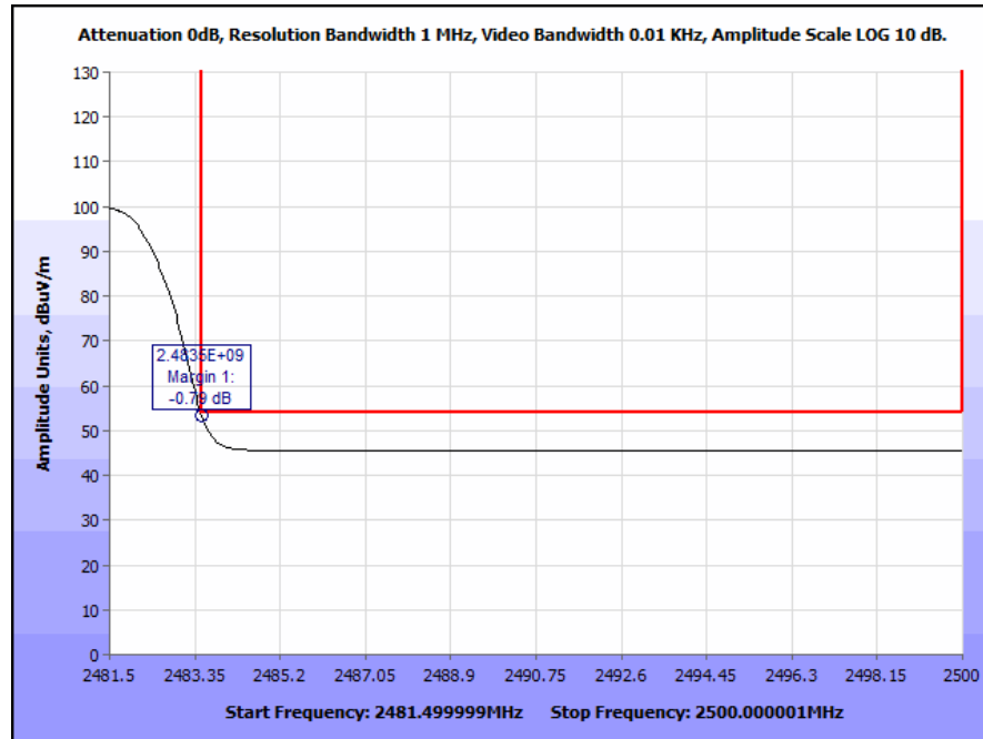
Plot 24. Radiated Restricted Band Edge, High Channel, Average
