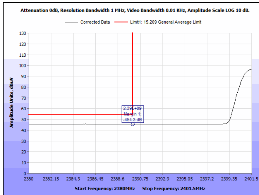
Plot 22. Radiated Restricted Band Edge, Low Channel, Average
