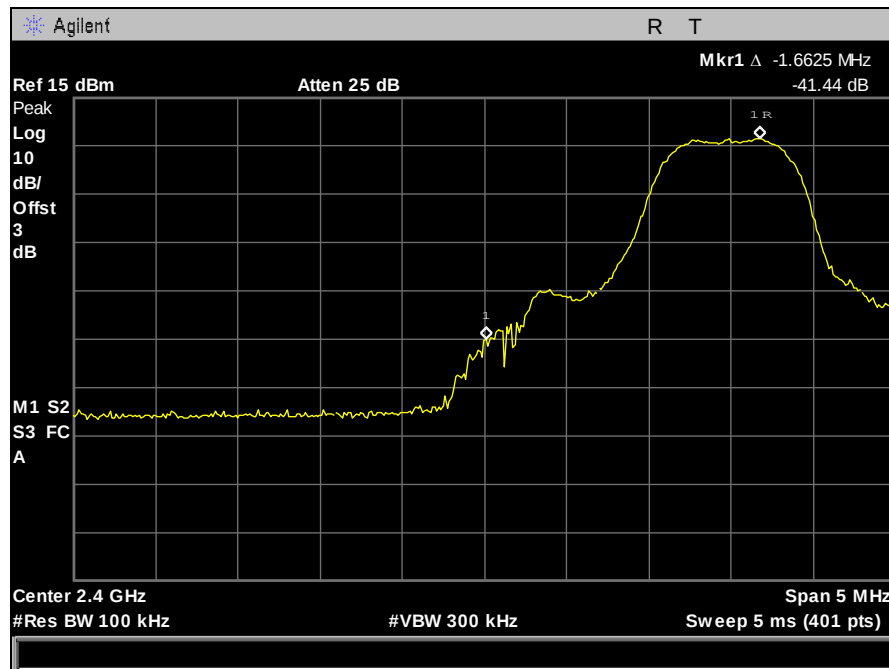
Plot 32. Conducted Band Edge, Low Channel
