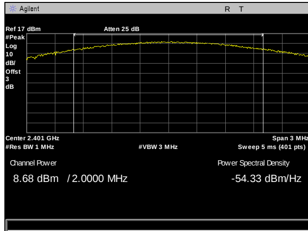
Plot 4. Peak Power Output, Low Channel, Integrated
