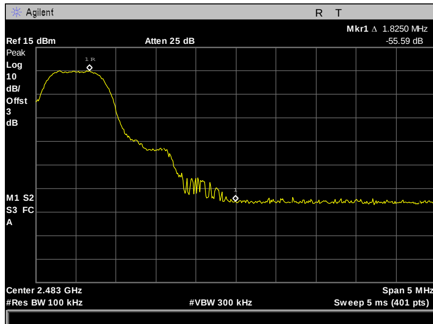
Plot 33. Conducted Band Edge, High Channel
