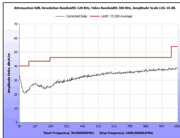
Plot 17. Radiated Spurious Emissions, High Channel, 30 MHz – 1 GHz
