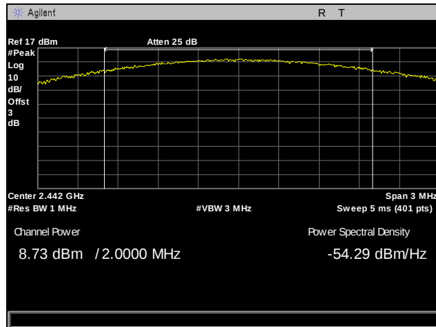
Plot 5. Peak Power Output, Mid Channel, Integrated
