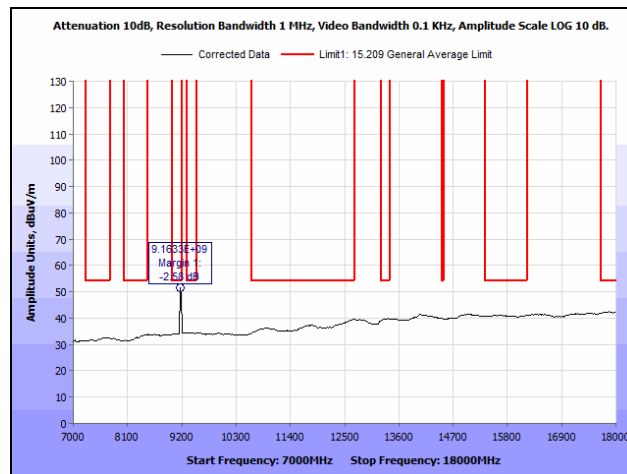
Plot 15. Radiated Spurious Emissions, Mid Channel, 7 GHz – 18 GHz, Average
