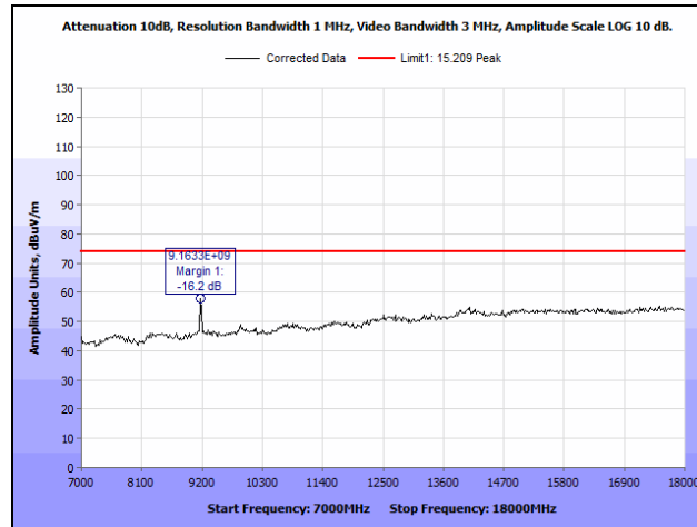
Plot 16. Radiated Spurious Emissions, Mid Channel, 7 GHz – 18 GHz, Peak
