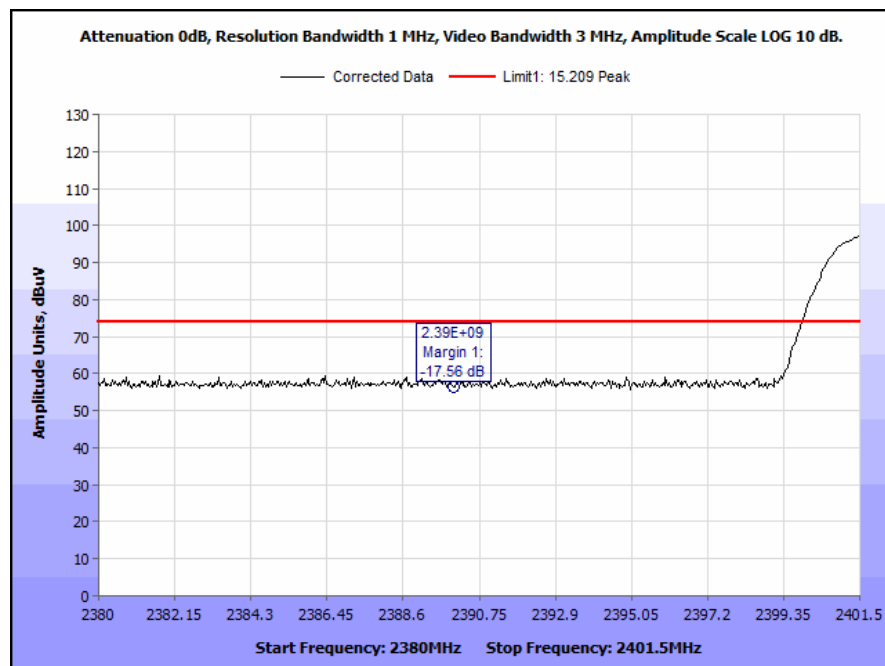
Plot 23. Radiated Restricted Band Edge, Low Channel, Peak
