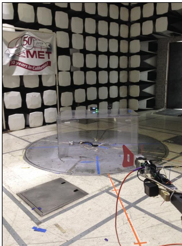
Photograph 3. Radiated Spurious Emissions, Test Setup, 2
