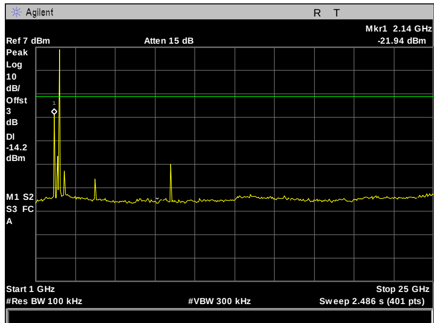
Plot 29. Conducted Spurious Emissions, Mid Channel, 1 GHz – 25 GHz
