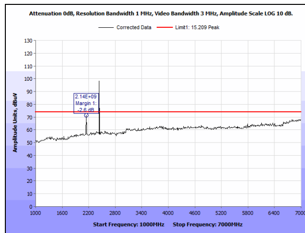
Plot 14. Radiated Spurious Emissions, Mid Channel, 1 GHz – 7 GHz, Peak
