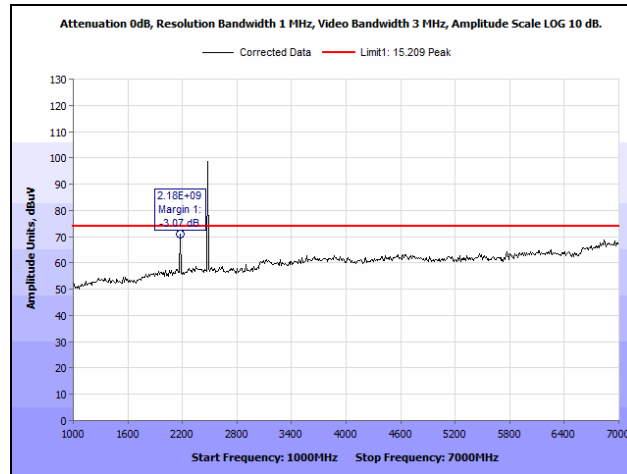
Plot 19. Radiated Spurious Emissions, High Channel, 1 GHz – 7 GHz, Peak
