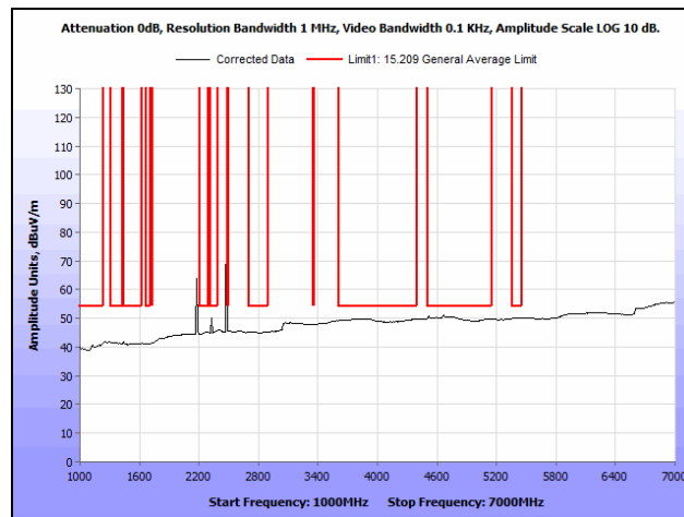
Plot 18. Radiated Spurious Emissions, High Channel, 1 GHz – 7 GHz, Average
