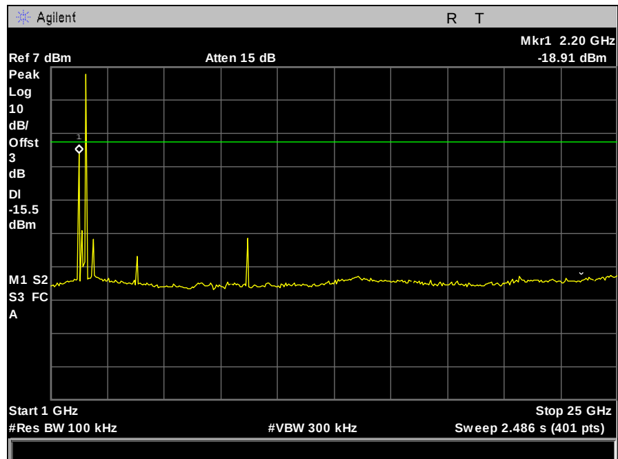
Plot 31. Conducted Spurious Emissions, High Channel, 1 GHz – 25 GHz
