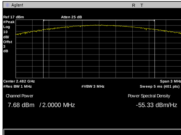
Plot 6. Peak Power Output, High Channel, Integrated
