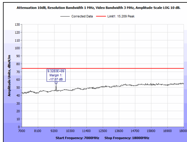
Plot 21. Radiated Spurious Emissions, High Channel, 7 GHz – 18 GHz, Peak
