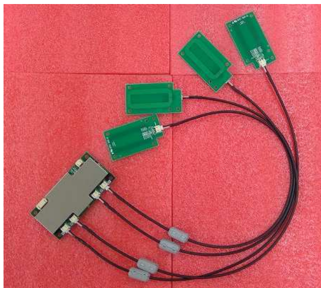
Connect the EUT and all external antenna
