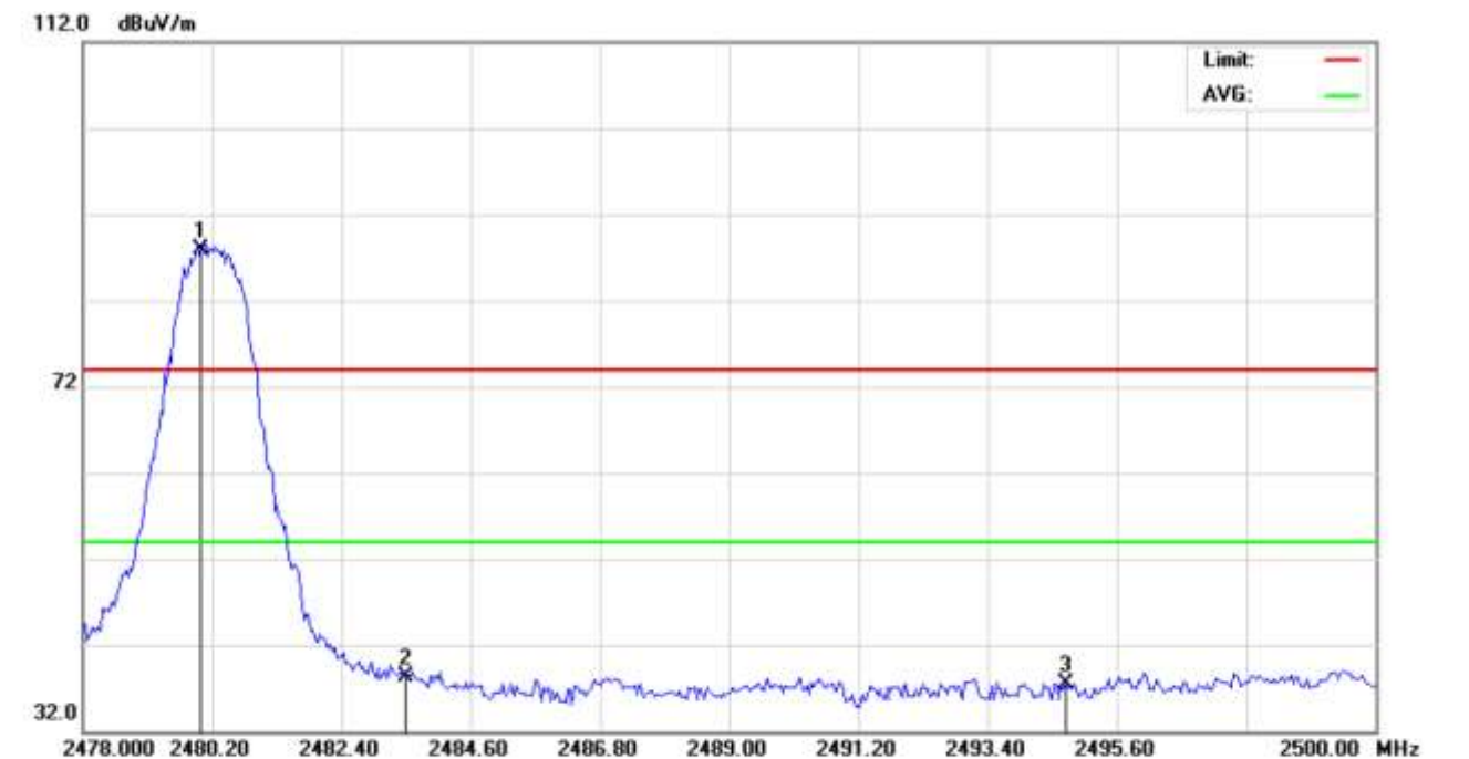
TEST PLOT OF BAND EDGE FOR HIGH CHANNEL (3Mbps)-Horizontal
