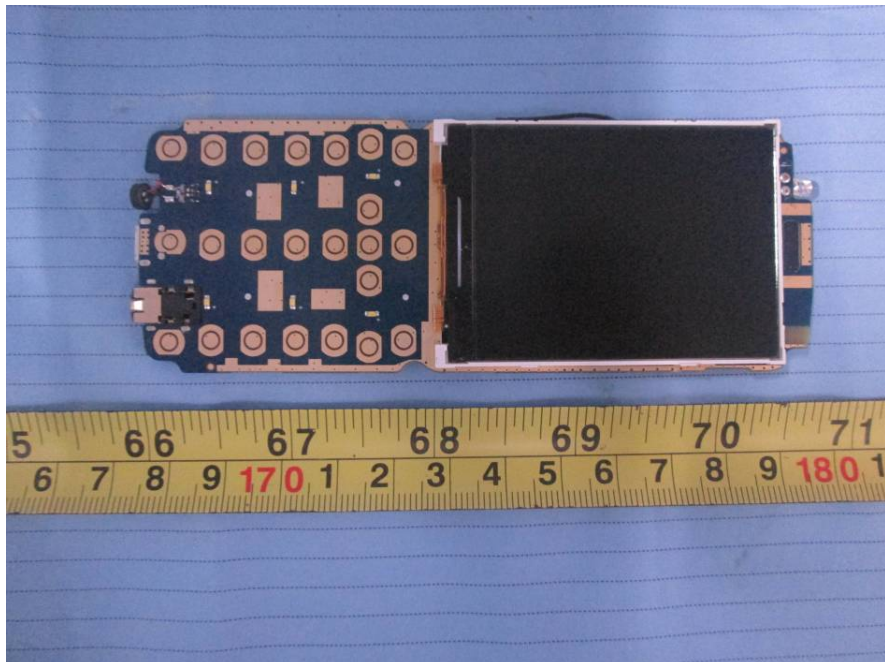
EUT – Main Board Back View 2
