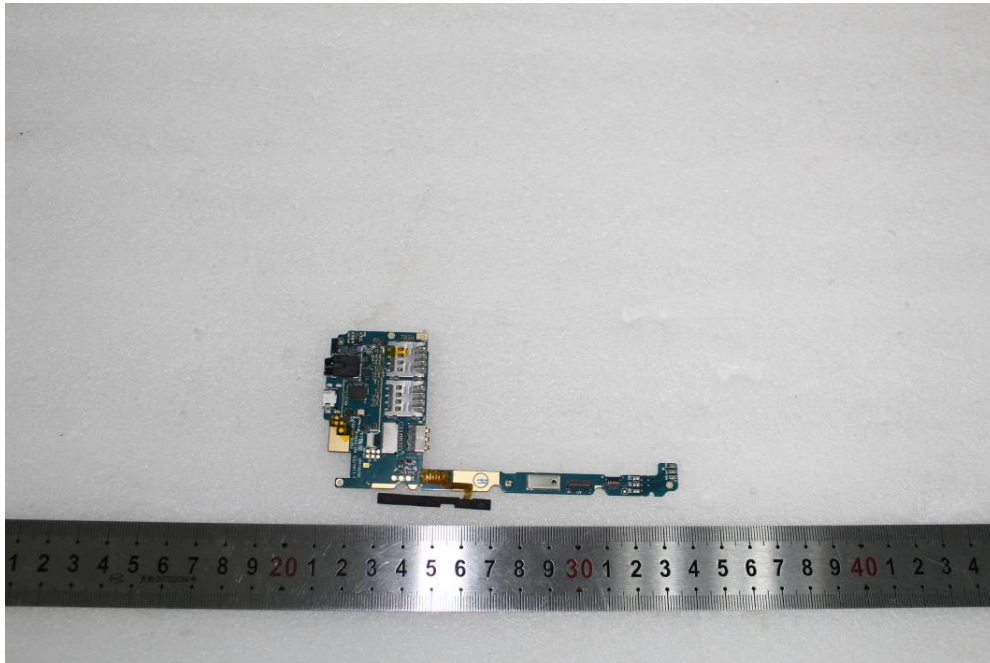
EUT – Main Board Front Shielding off View
