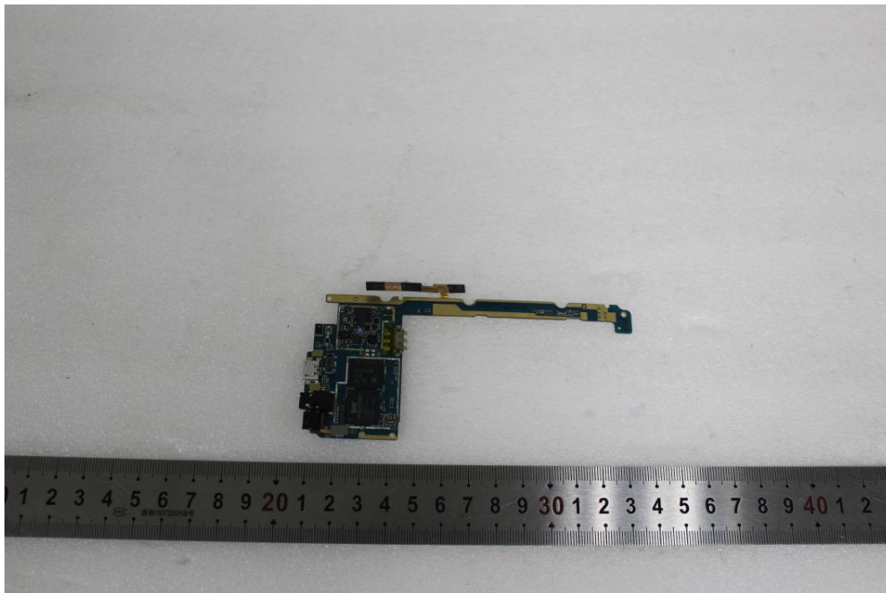
EUT – Main Board Rear Shielding off View
