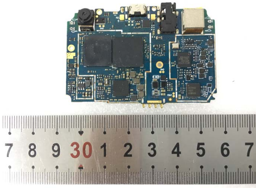
EUT – Mainboard Top 1 Shielding off View
