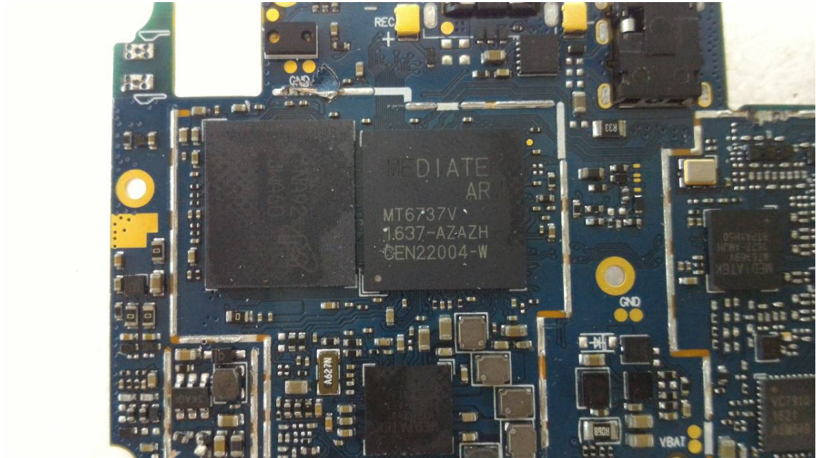
EUT – IC Chip View 1
