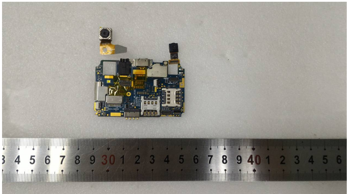
EUT – Mainboard 1 Cover off View
