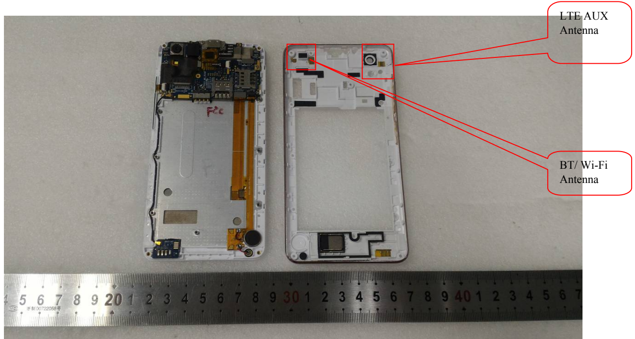
EUT – Cover off View 2
