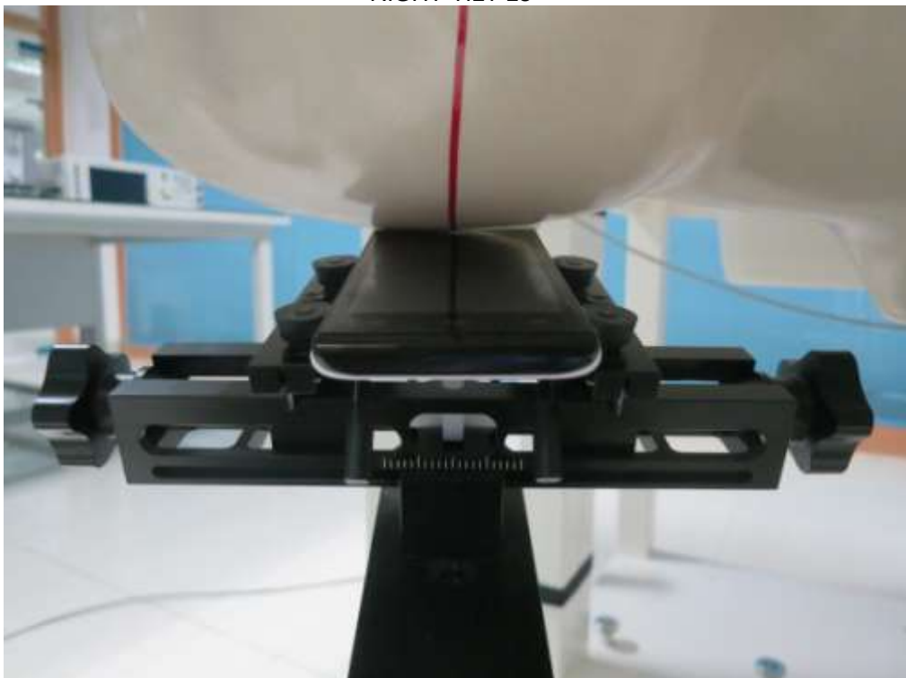
RIGHT-TILT 15^{\circ}
