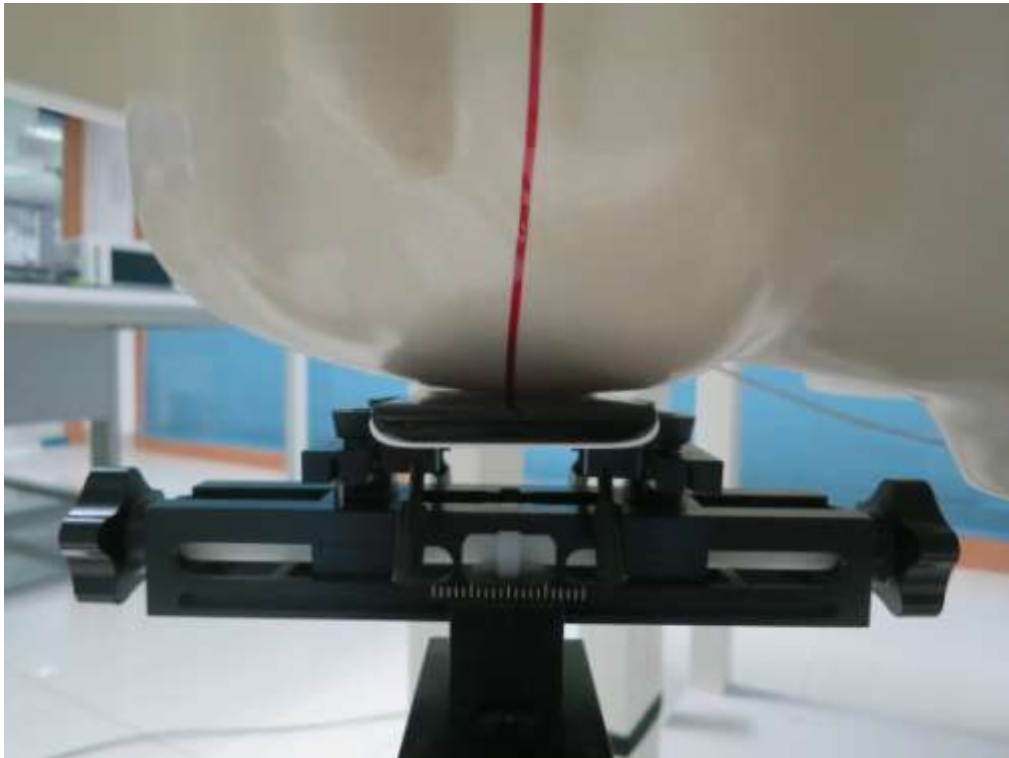
RIGHT-TILT 15^{\circ}
