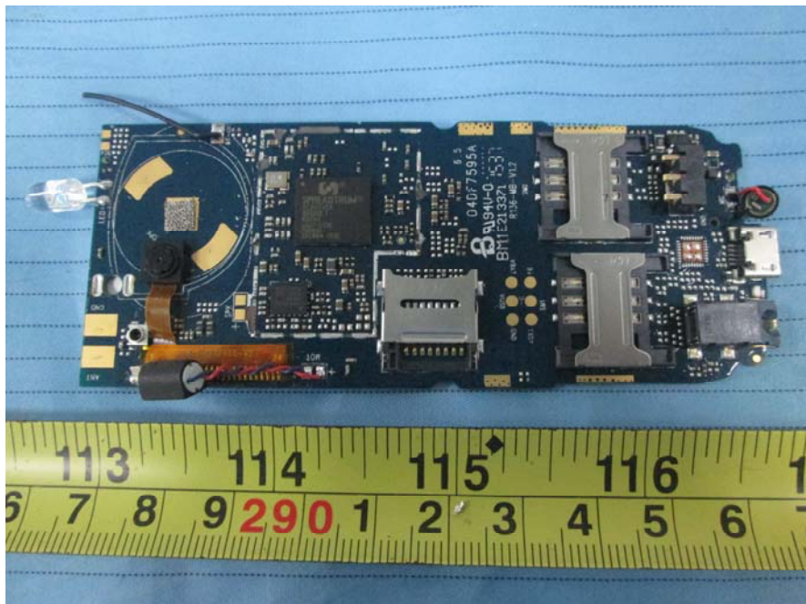
EUT – Unshielded Mainboard View
