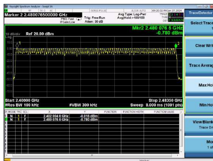
8-DPSK Modulation
