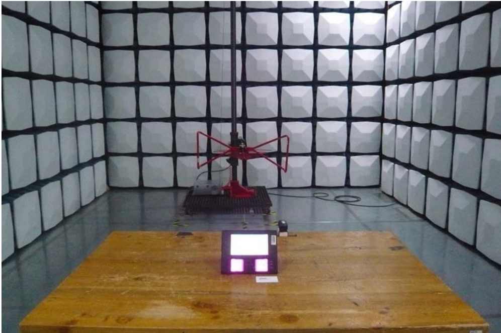
Radiated Emissions 30MHz-1GHz - View
