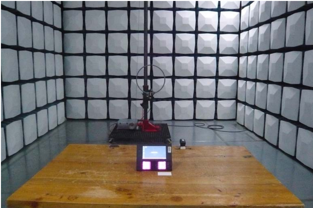
Radiated Emission 9 KHz-30 MHz –View
