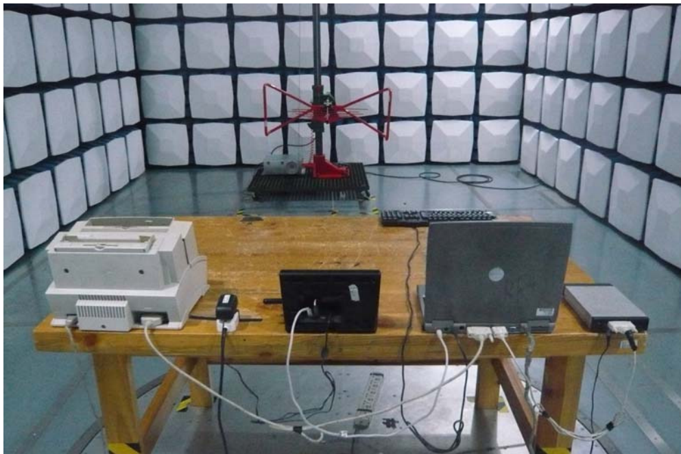
Radiated Emissions Below 1GHz –Rear View
