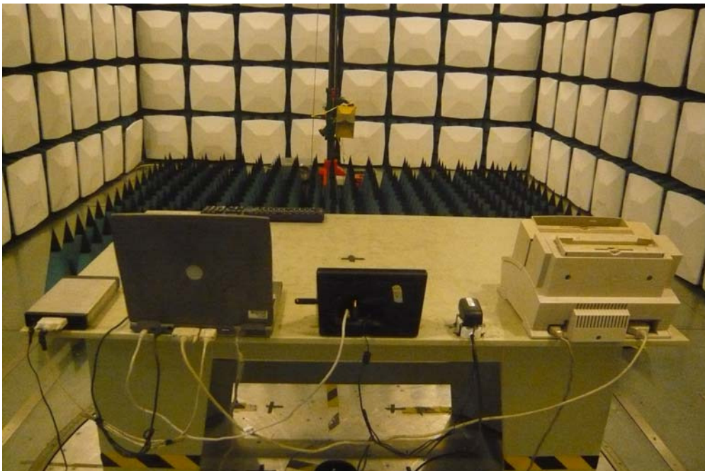
Radiated Emissions Above 1GHz –Rear View
