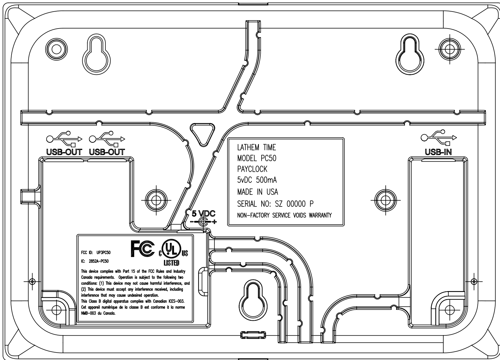
PC50 ENCLOSURE- REAR VIEW
