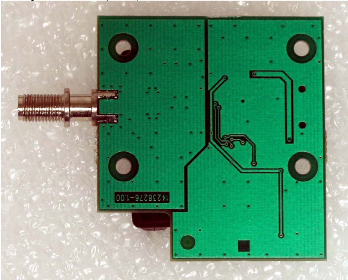
Exchangeable RF Module (Bottom):
