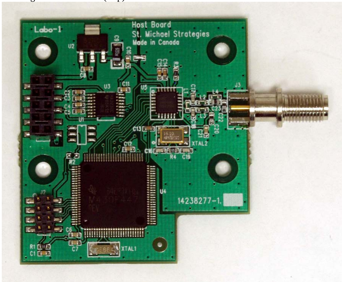
Exchangeable RF Module (Top):
