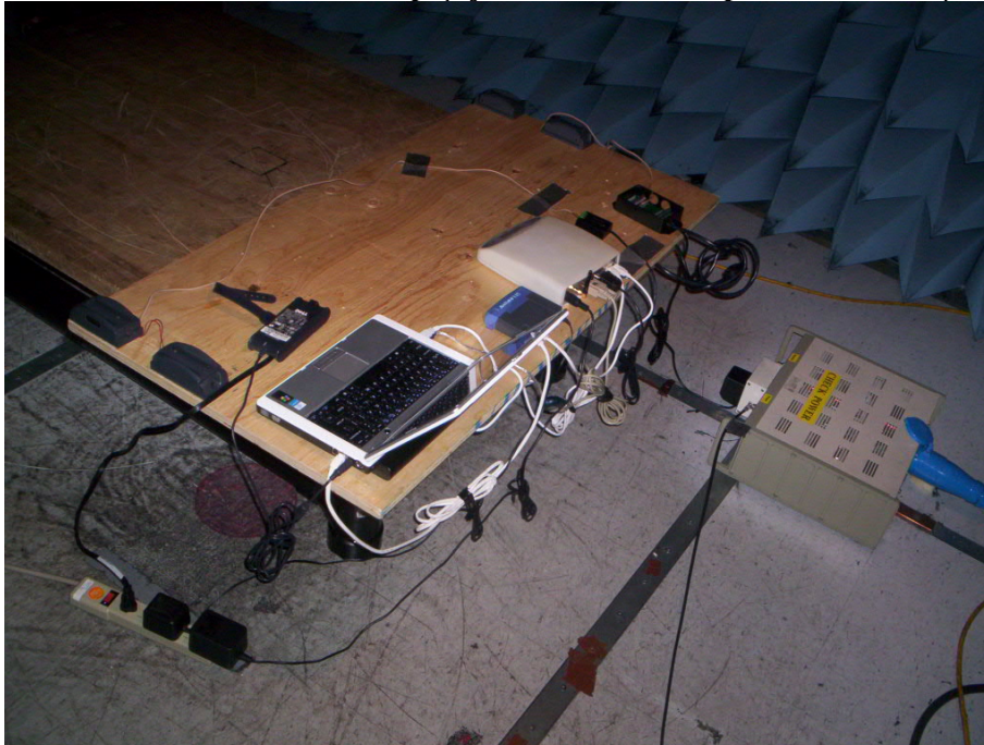
Conducted Emissions Setup (System, Normal Operation Mode):
