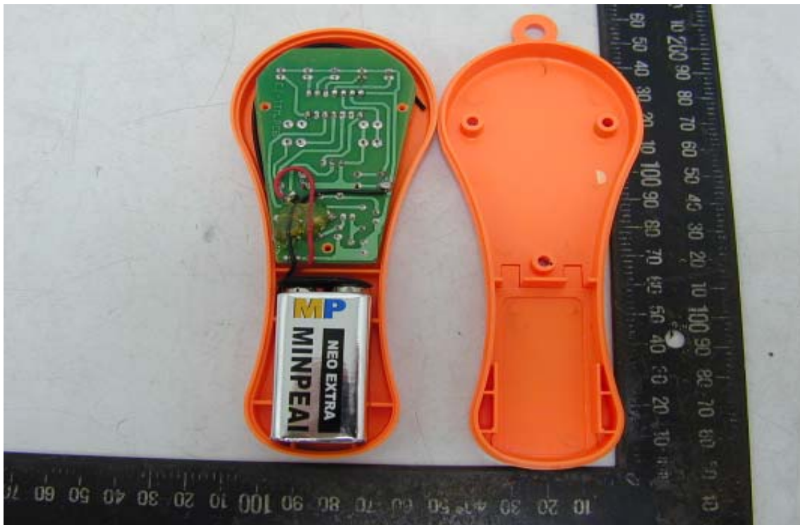
Inside View of Remote Controller
