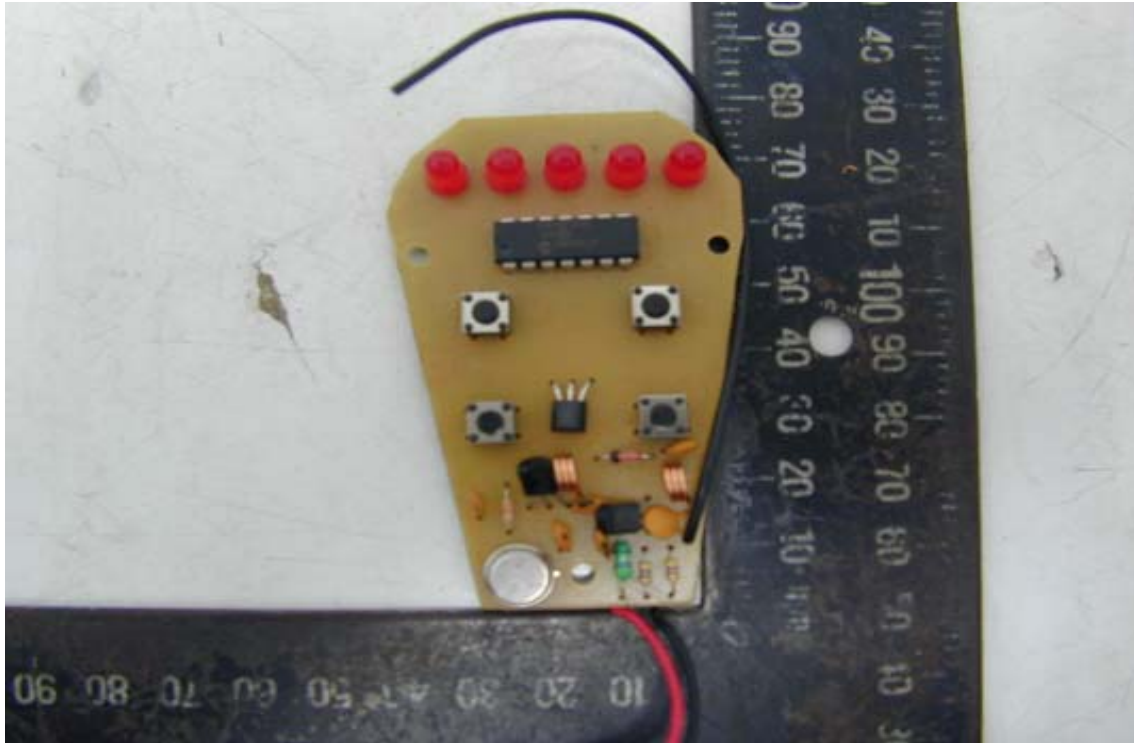
Component Side of Main Board of Remote Controller
