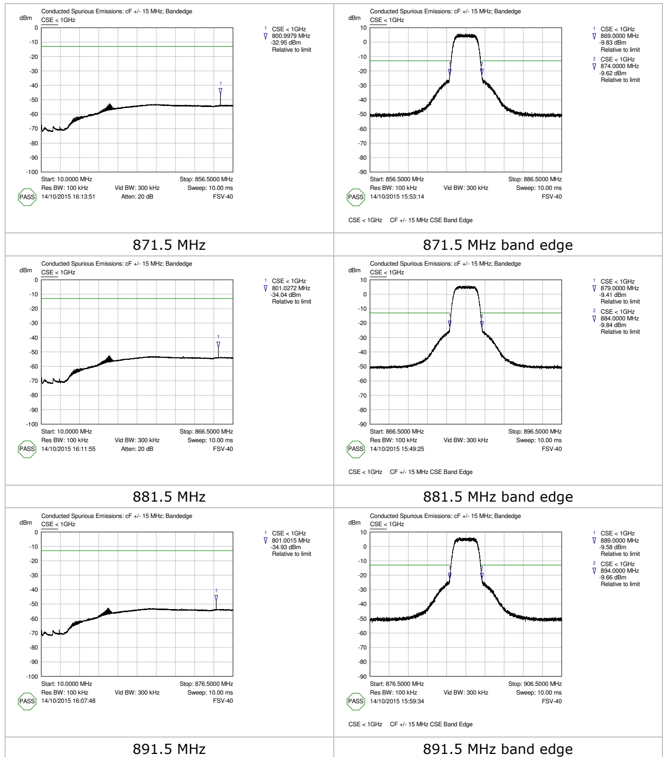
Figure 8: Wideband CSE inc. band edge
