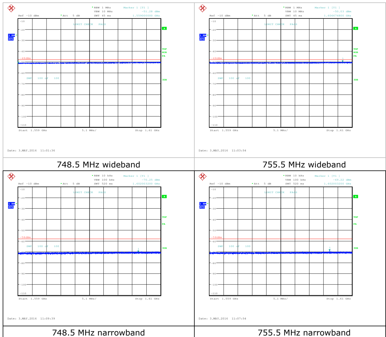
Figure 11: Emissions in the band 1559-1610 MHz
