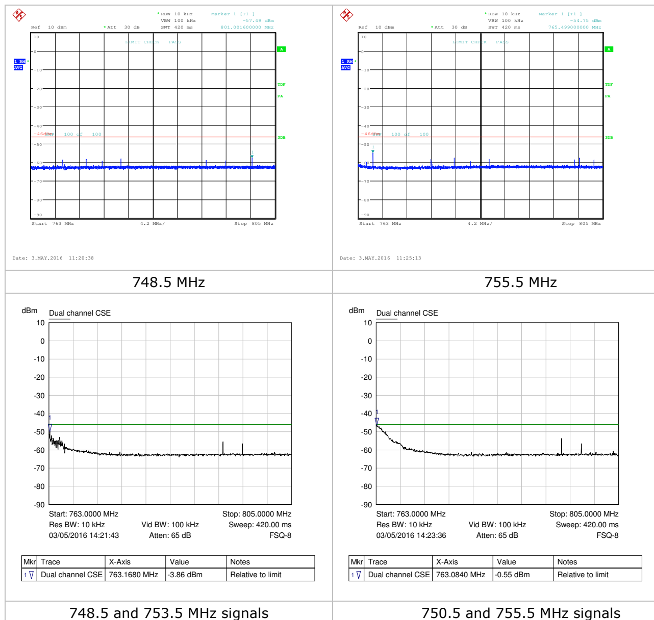
Figure 10: Emissions between 763-775 MHz and 793-805 MHz
