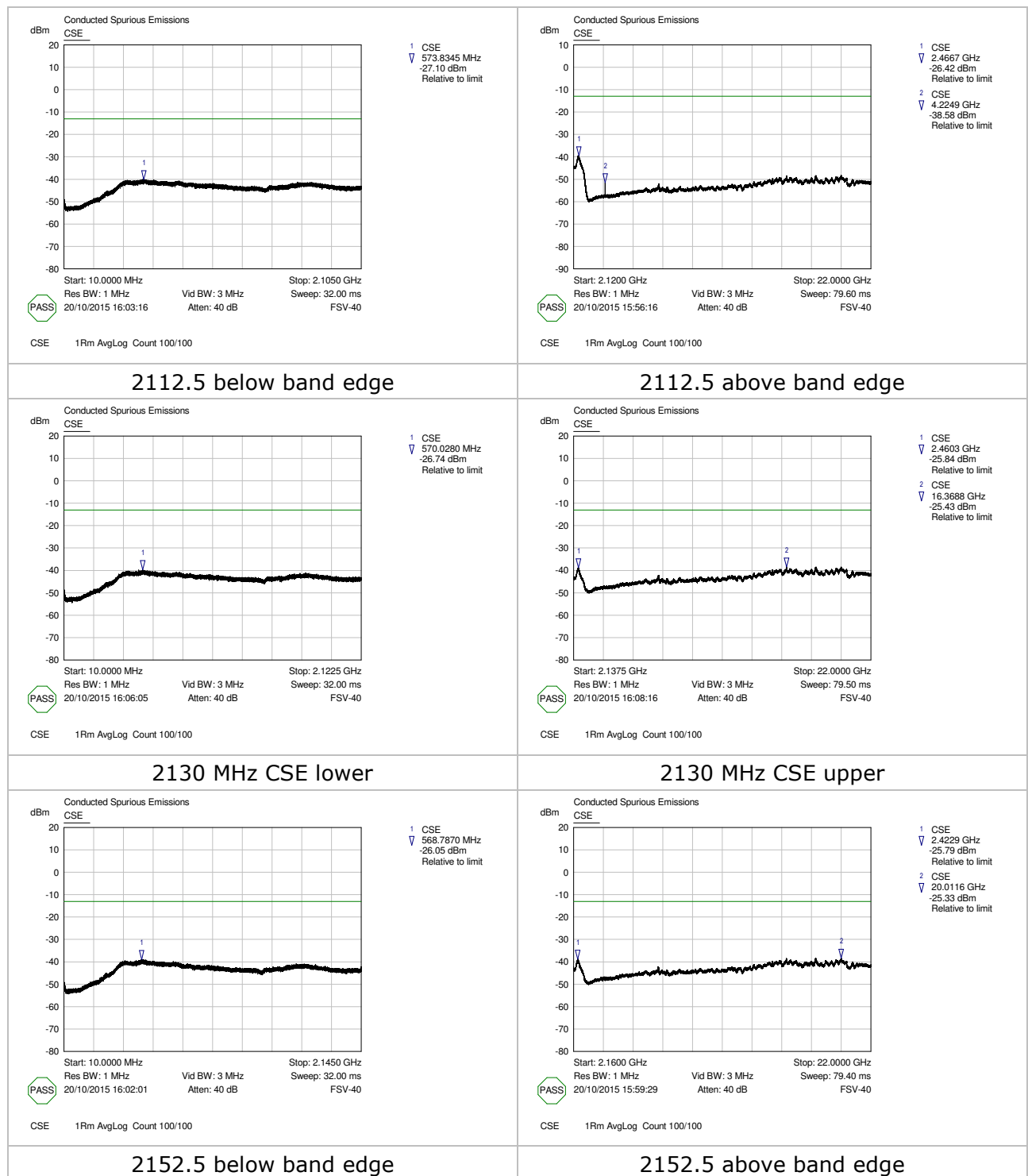
Figure 15: CSE except band edge 2110-2155 MHz Band
