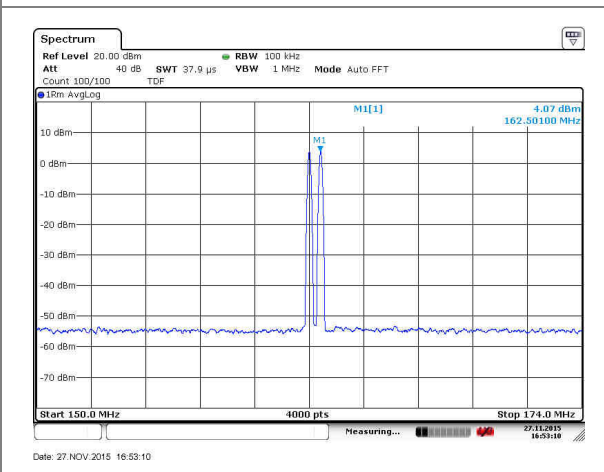
Figure 4: Multi-channel transmit power and intermodulation
