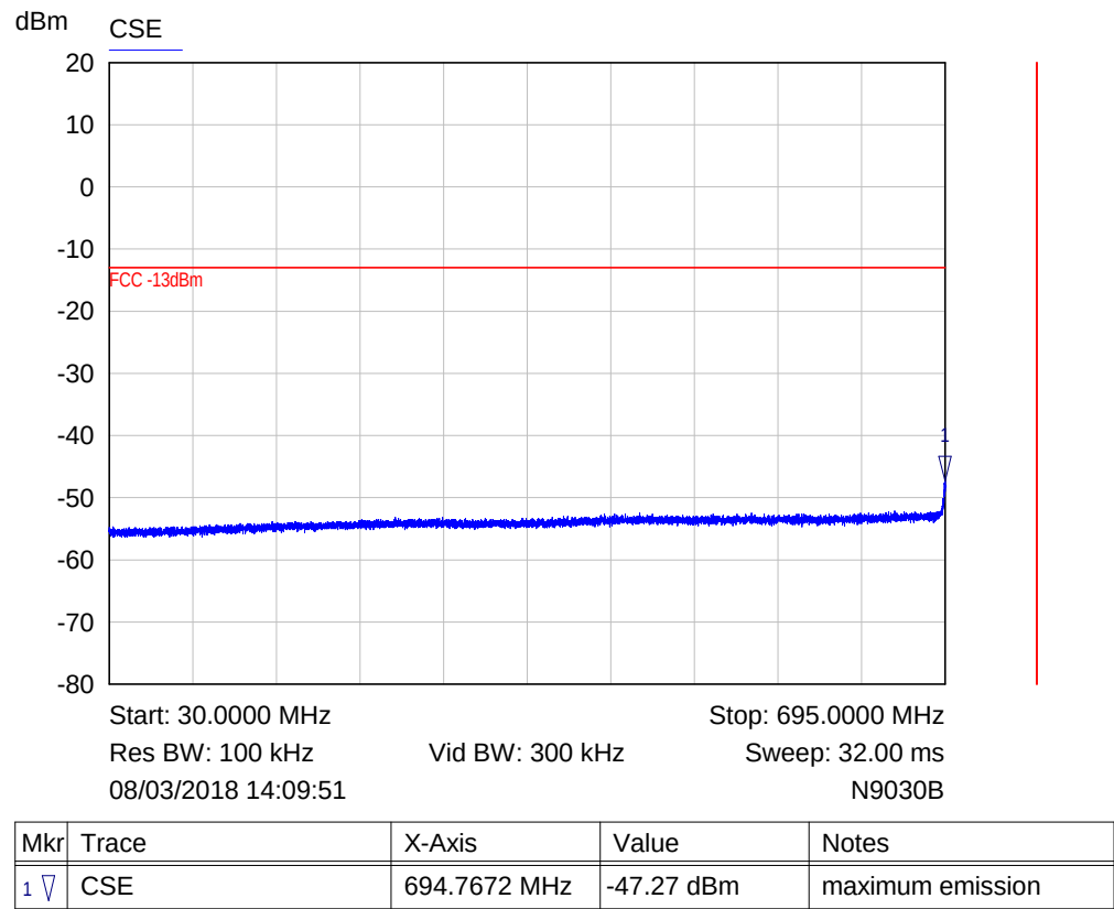
Plot of conducted emissions single Low channel (700.5MHz) 30 – 695 MHz range
