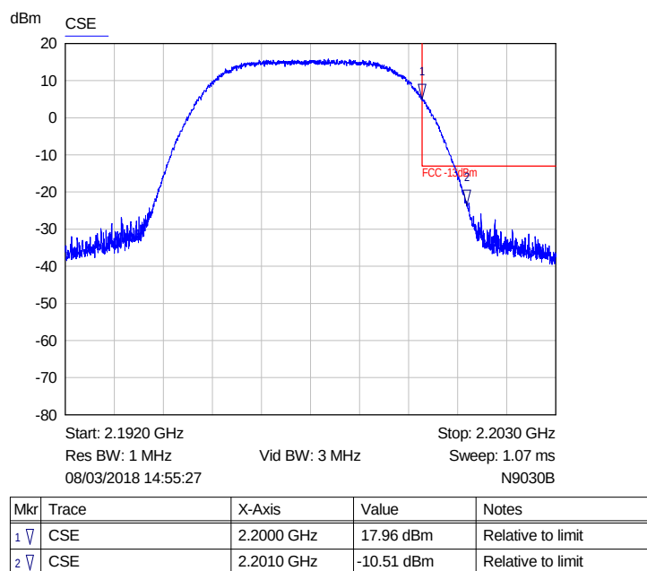
Plot of upper band edge for High channel 1MHz RBW (2197.5MHz)
