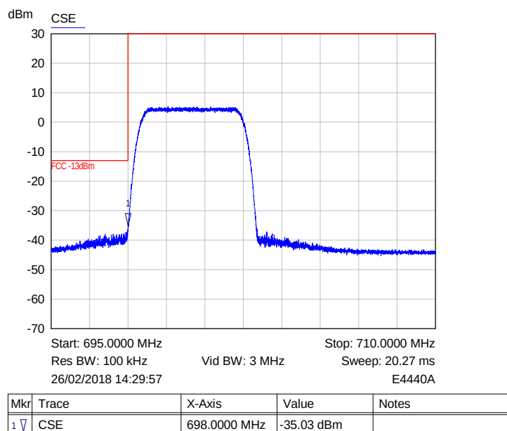
Plot of lower band edge for Low channel (700.5MHz)
