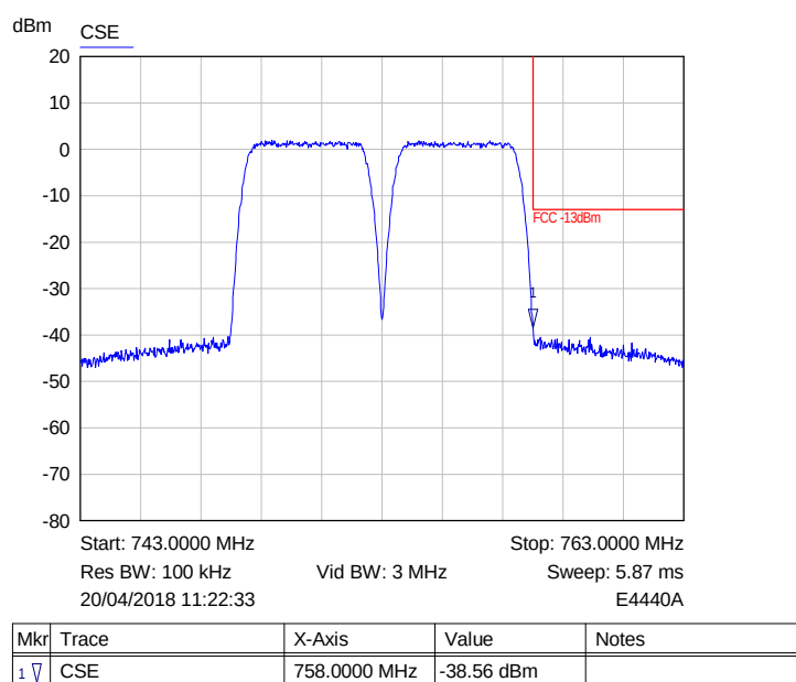
Plot of upper band edge for High channels (750.5 & 755.5MHz)
