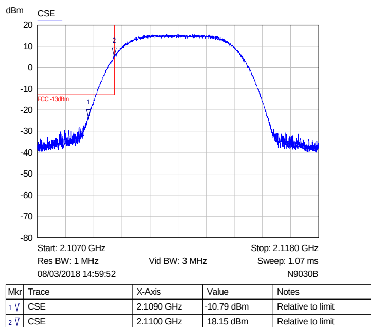
Plot of lower band edge for Low channel 1MHz RBW (2112.5MHz)
