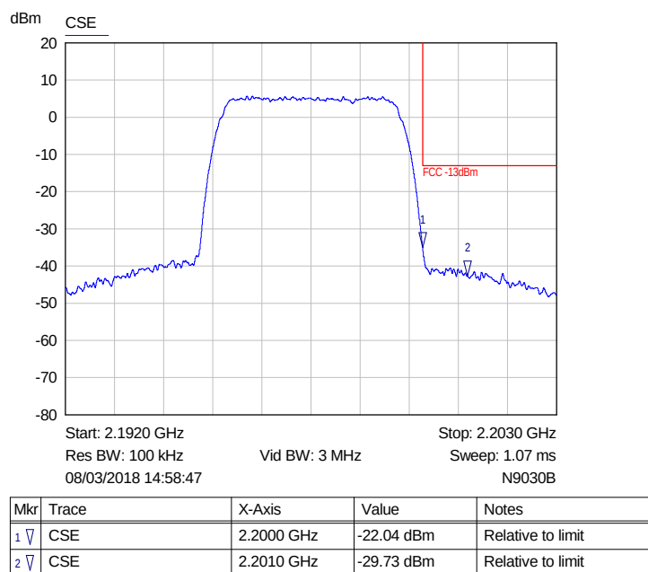
Plot of upper band edge for High channel 100kHz RBW (2197.5MHz)
