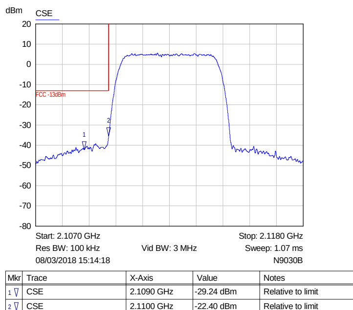
Plot of lower band edge for Low channel 100kHz RBW (2112.5MHz)
