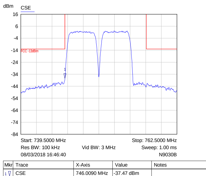
Plot of lower band edge for Low channels (748.5 & 753.5MHz)
