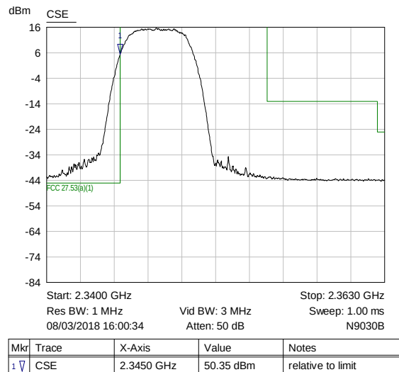
Plot of lower/upper band edge for Low channel 1MHz RBW (2347.5 MHz)
