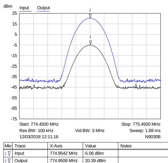
Plot of Channel power at determined f_0 in Band 769-775 MHz
