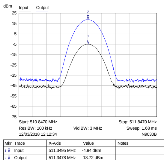
Plot of Channel power at determined f_0 in Band 456-512 MHz
