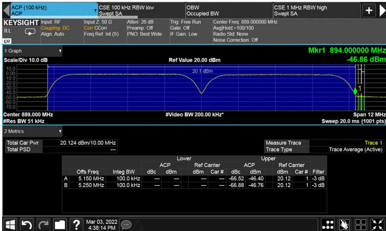
Plot of upper band edge for High channels (886.5 & 891.5 MHz)
