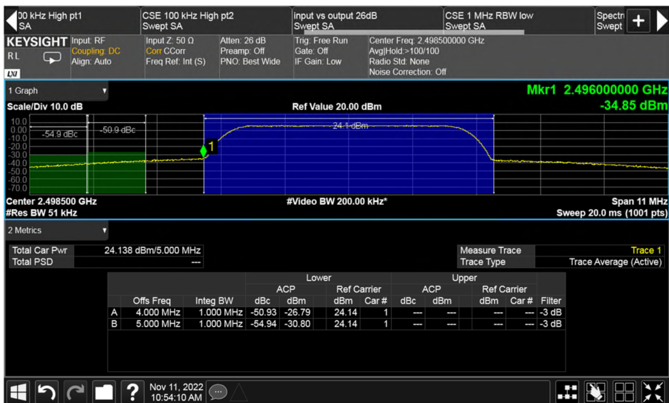
Plot of lower band edge for Low channel (2498.5MHz)
