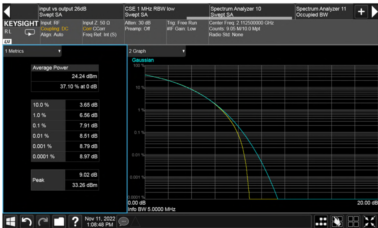
Plot of Peak to Average power ratio at determined f_0 in band 2110-2180 MHz
