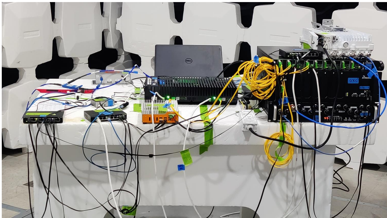
Figure 2 – Band 48 Radiated Spurious Emission Test Set Up: 30MHz – 1GHz
